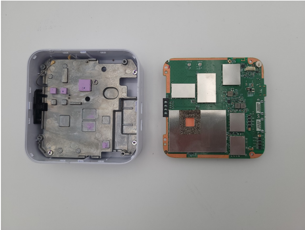
Photograph 5: Bottom of PCB Out of Top of DUT
