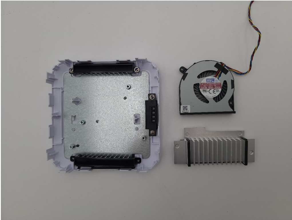
Photograph 3: Bottom Fan Removed
