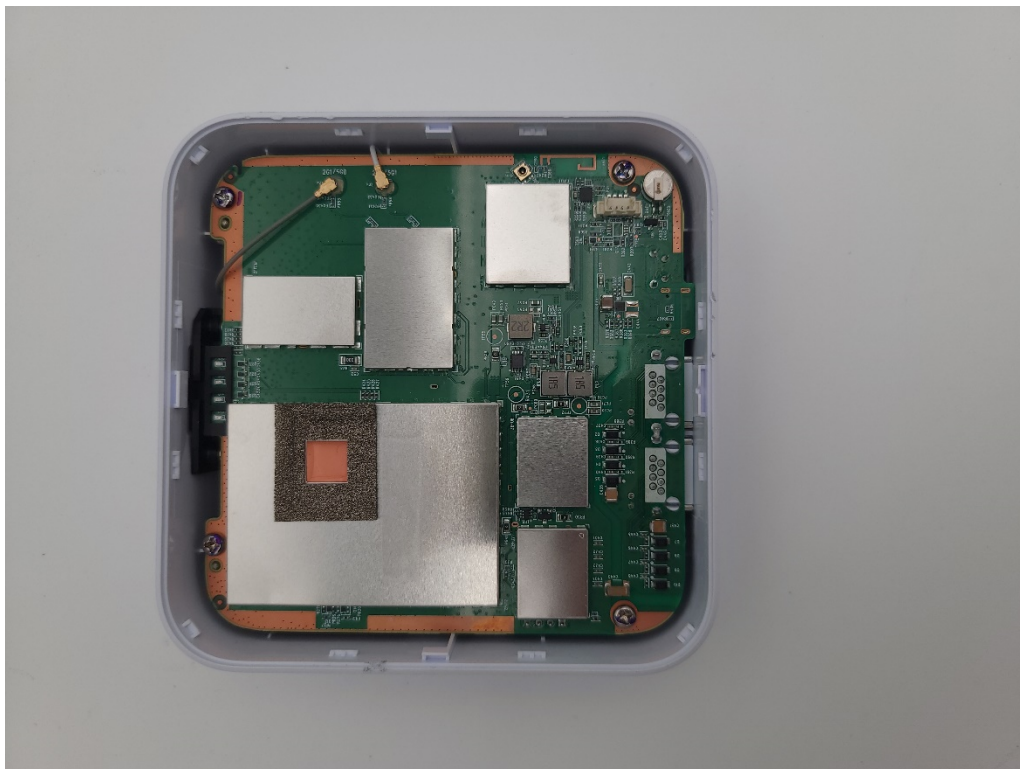
Photograph 4: Bottom of PCB in Top of DUT
