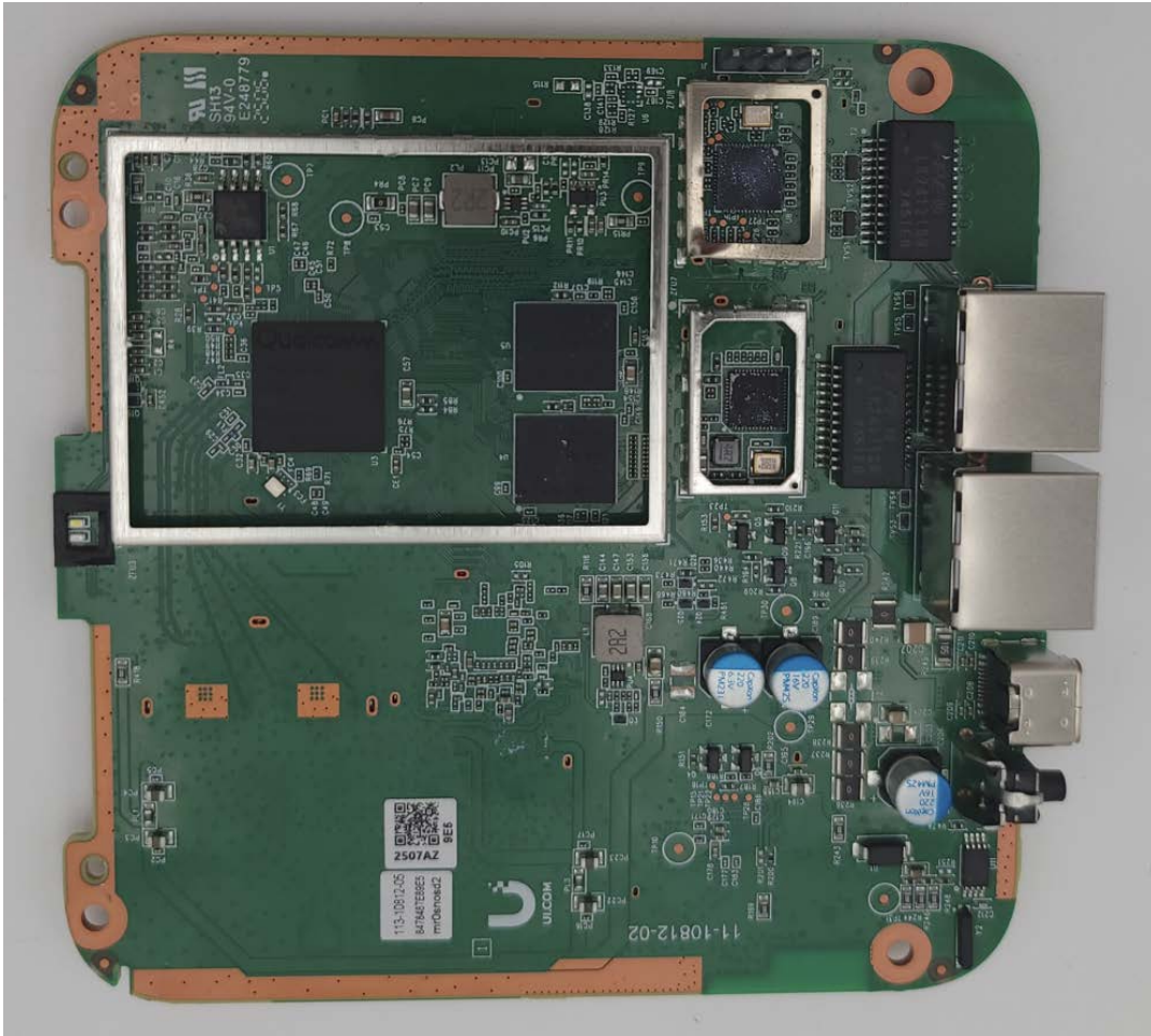
Photograph 2: Top of Main PC w/o Cans
