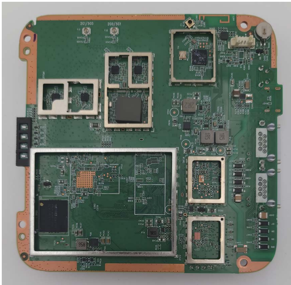
Photograph 4: Bottom of Main PC w/o Cans
