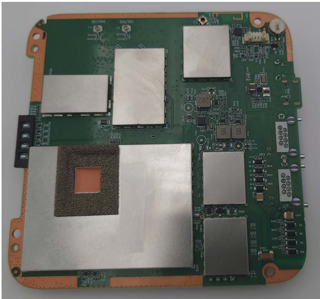
Photograph 3 Bottom of Main PC w/ Cans
