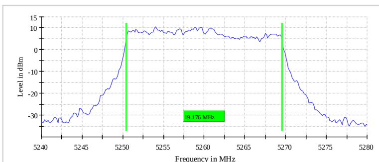
99 % Bandwidth
