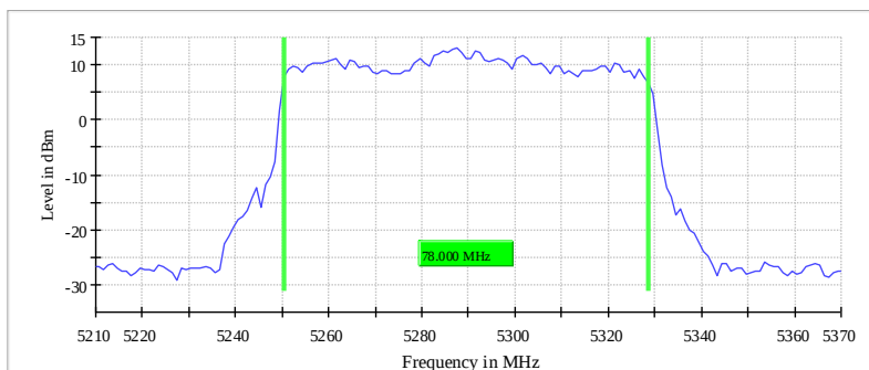
99 % Bandwidth
