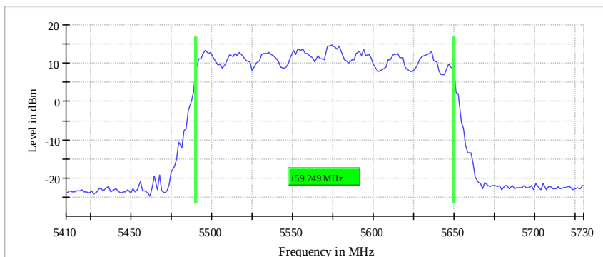
99 % Bandwidth
