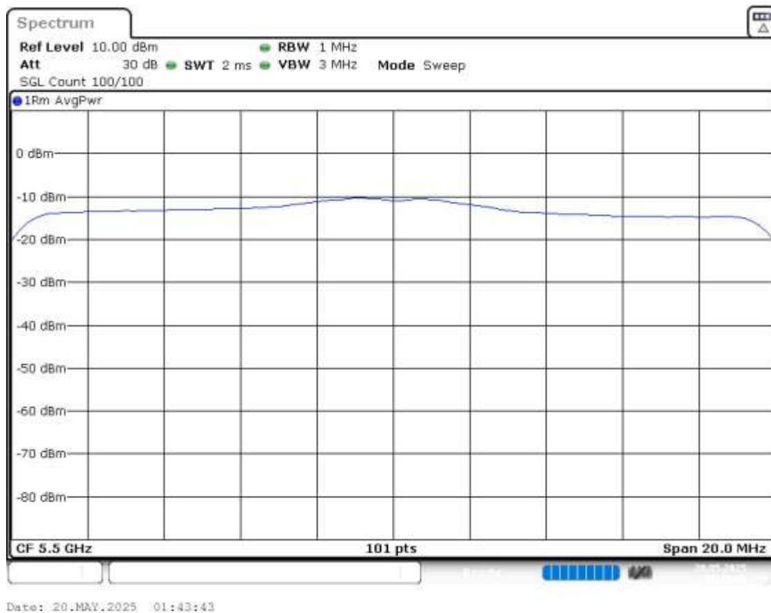
PSD Connector 1
