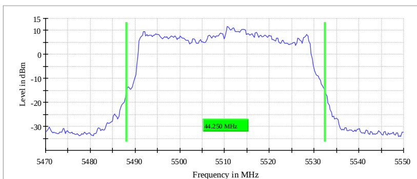
26 dB Bandwidth
