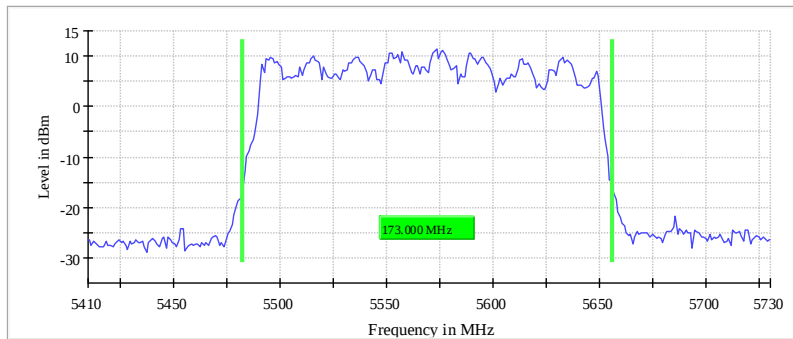
26 dB Bandwidth
