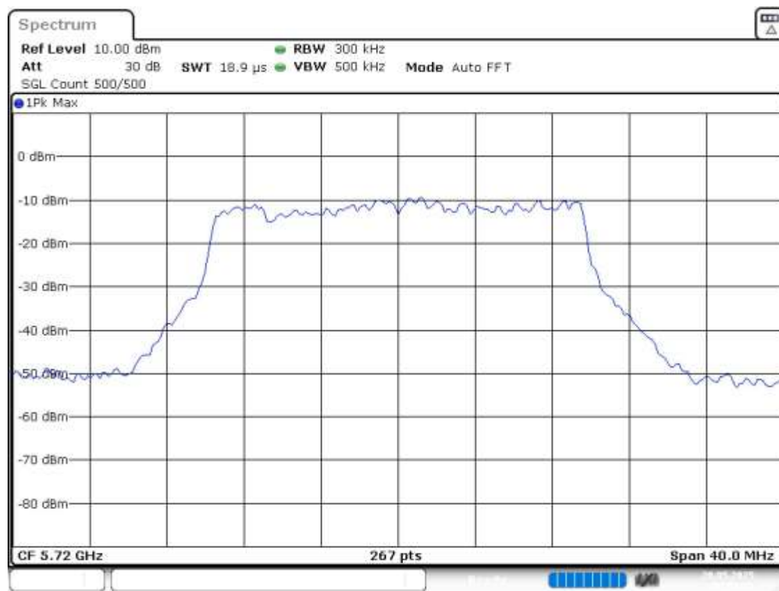
Bandwidth
