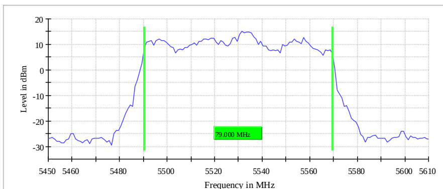
99 % Bandwidth
