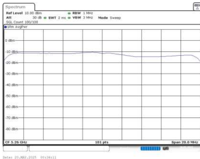
PSD Connector 1
