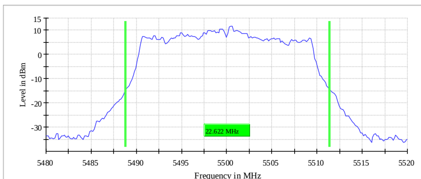
26 dB Bandwidth
