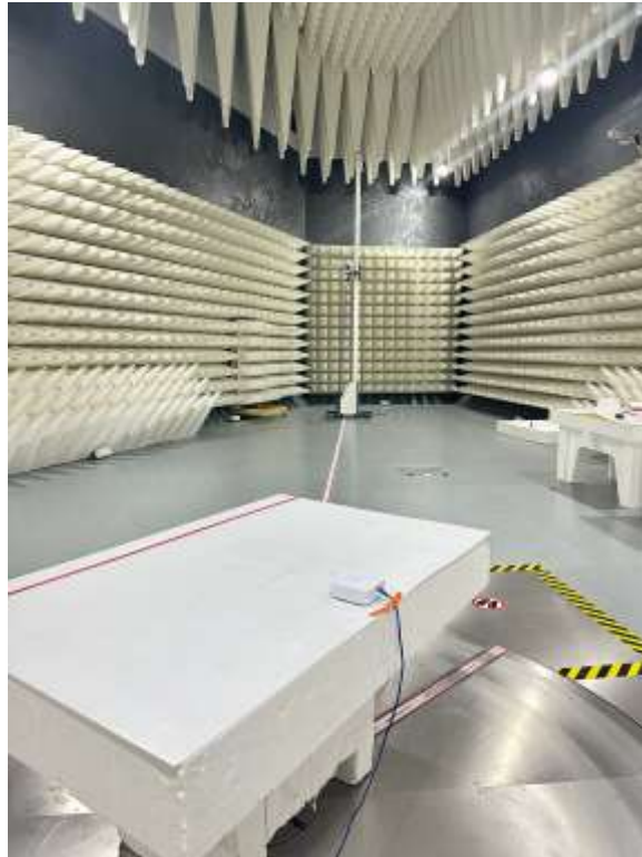
Photograph 1: View Test Set Up Radiated Emissions 30 – 1000 MHz
