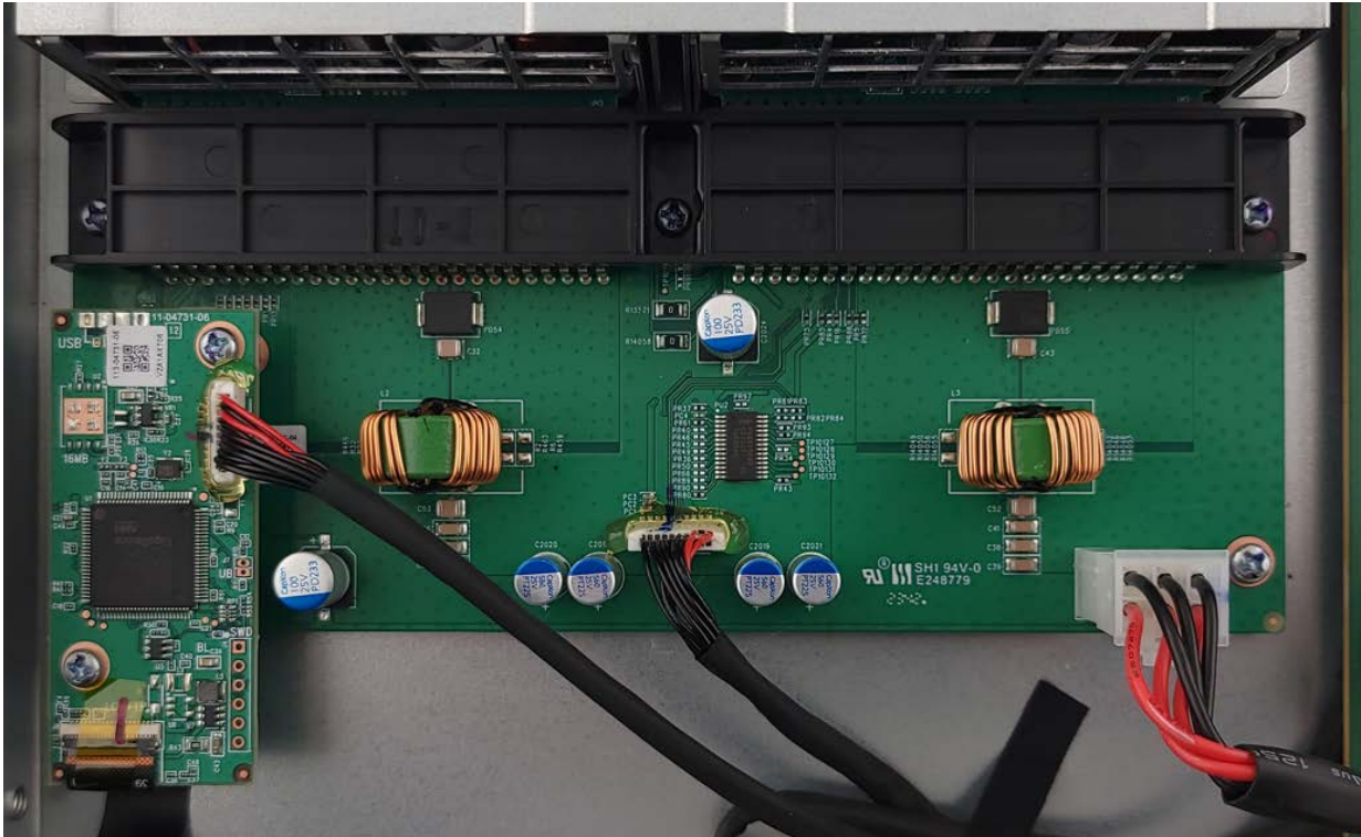
Photograph 4: Power Supply PCB
