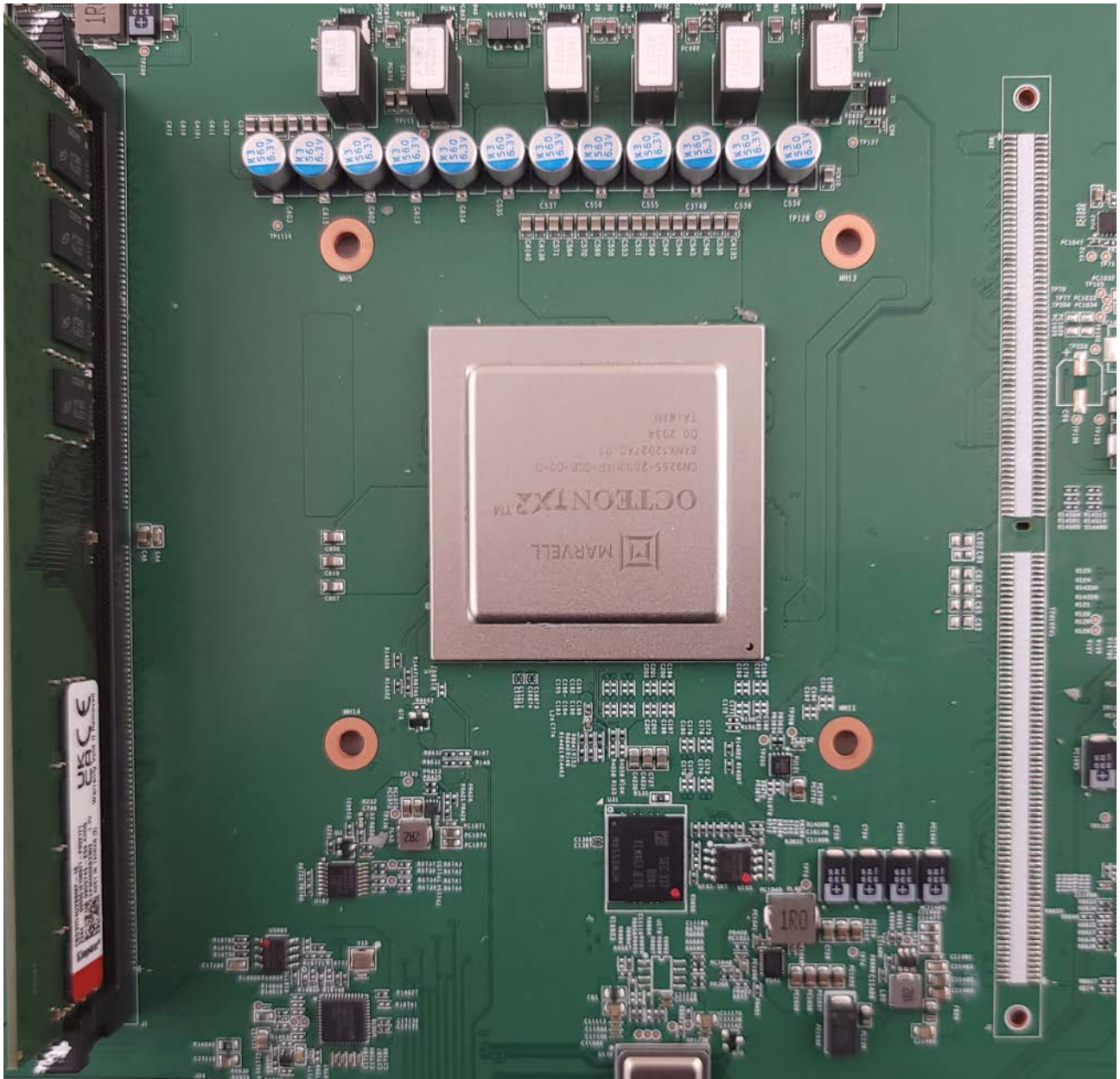
Photograph 1: Top of Main PCB with Heat Sink Off
