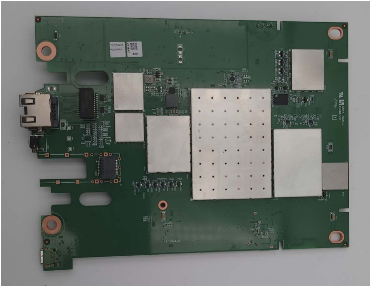
Photograph 12: Back of Main PCB with Cans
