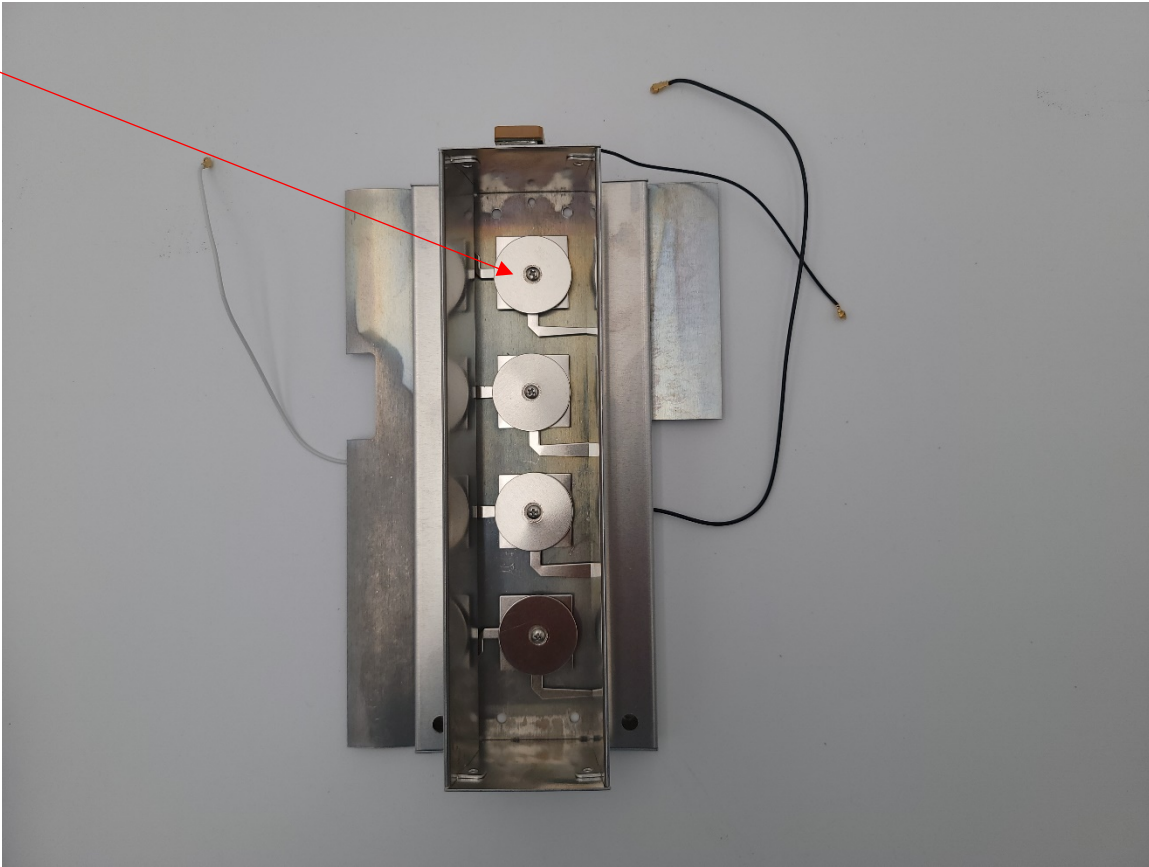
Photograph 7: 5 GHz Antenna Board
