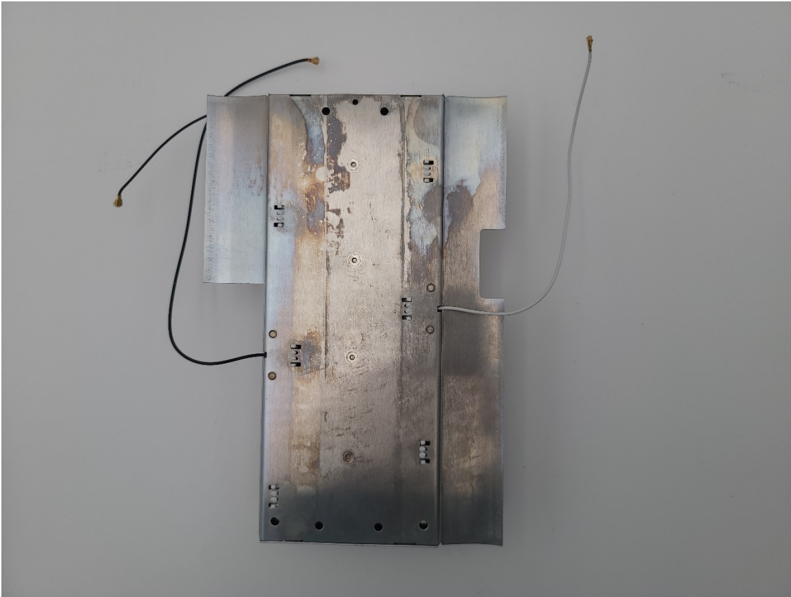
Photograph 8: Back of 5 GHz Transmitter Board
