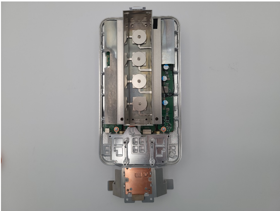
Photograph 3: 60 GHz Transmitter Mount Removed
