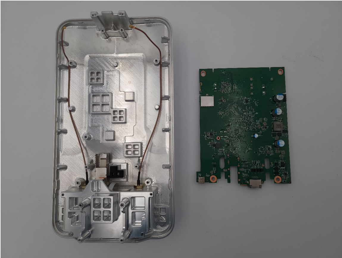
Photograph 9: Main PCB Removed from Back of DUT
