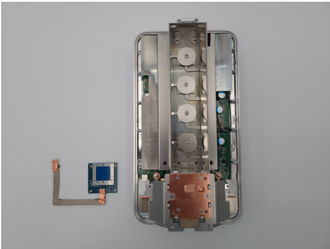
Photograph 2: 60 GHz Transmitter Removed
