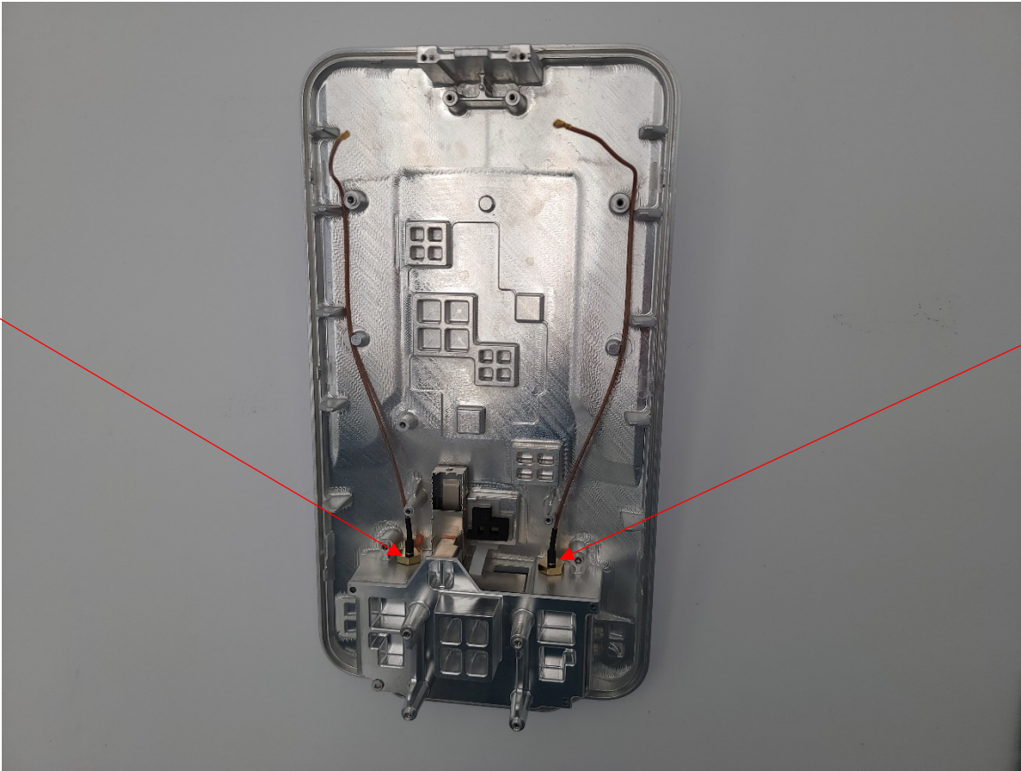
Photograph 10: Back of DUT with External Antenna Connections
