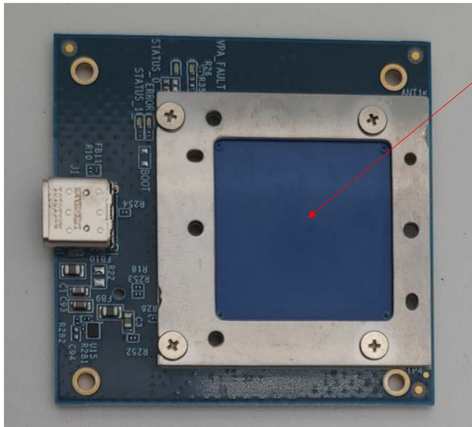
Photograph 4: 60 GHz Transmitter Board
