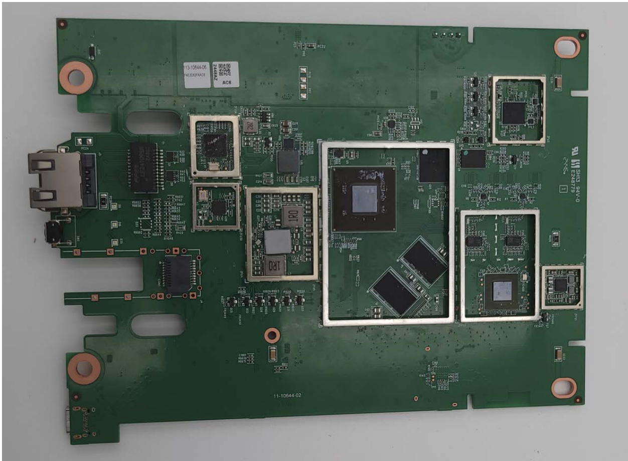
Photograph 2: Back of Main PCB with Cans Removed
