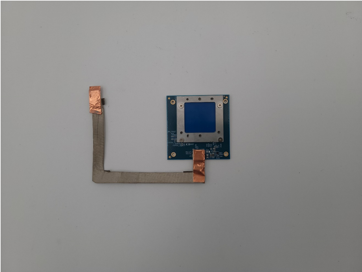
Photograph 3: 60 GHz Transmitter Board
