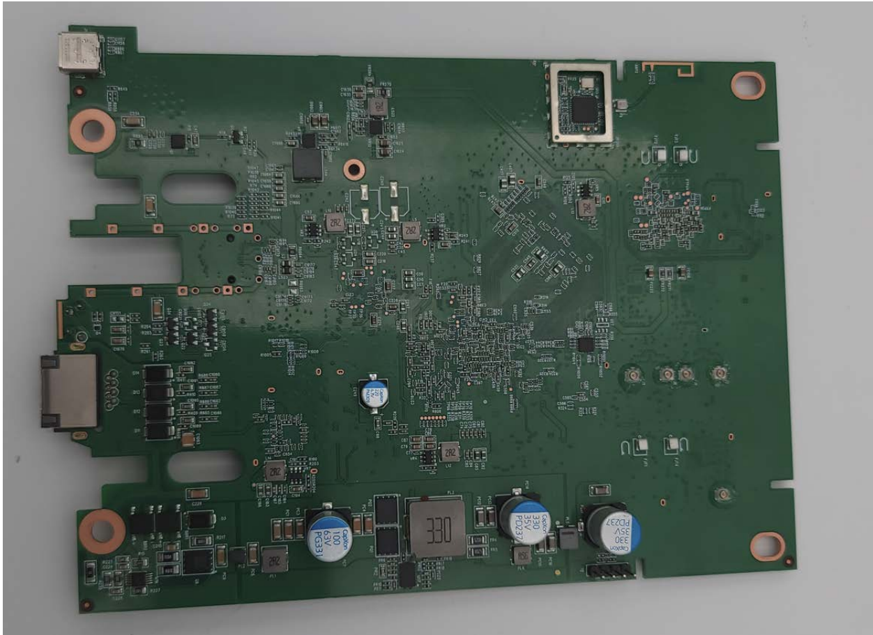
Photograph 1: Front of Main PCB with Can Removed
