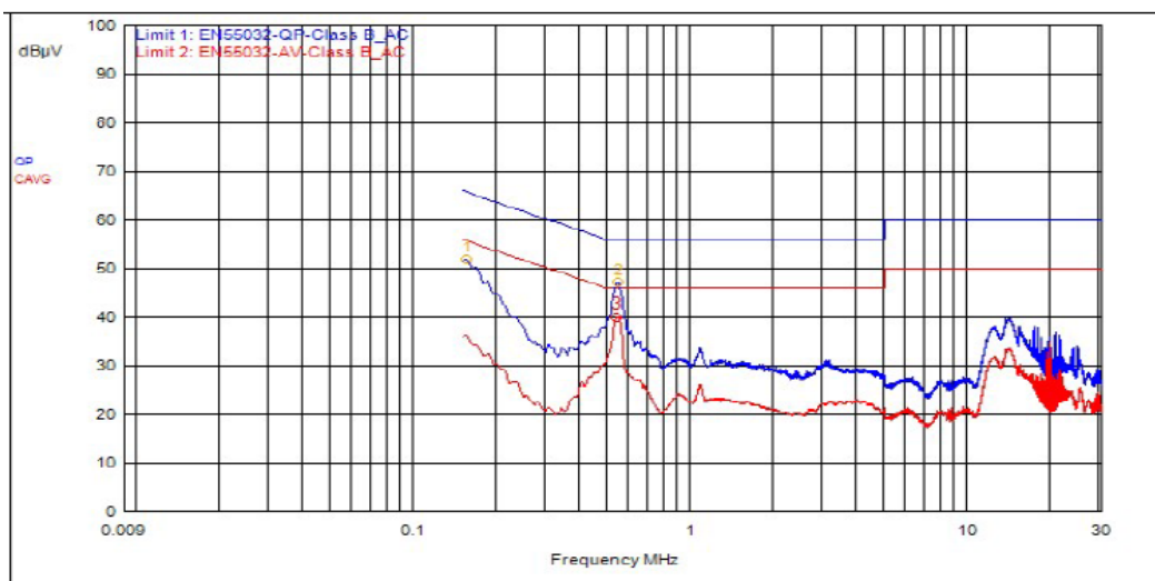
Graph 2: Conducted Emissions Plot - Line 1
