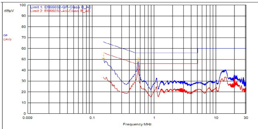
Graph 1: Conducted Emissions Plot - Neutral
