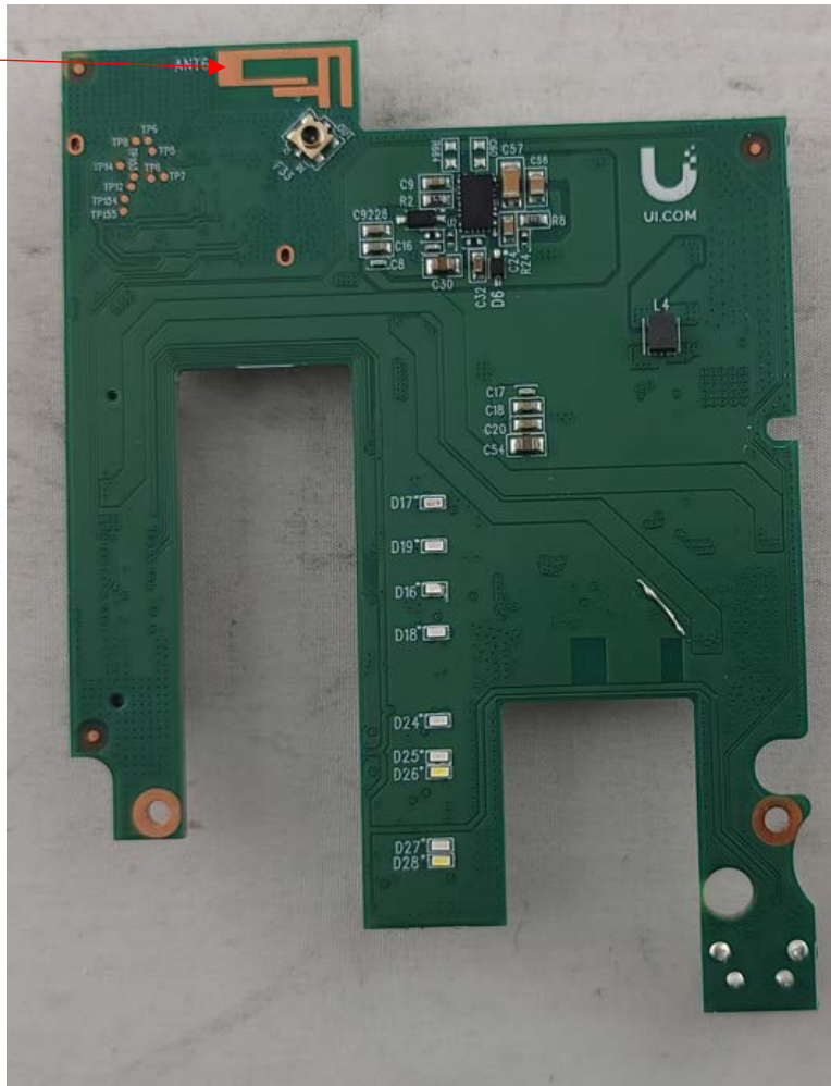
Photograph 4: Daughter Card Bottom
