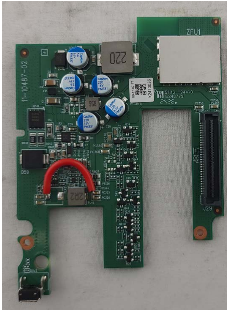
Photograph 3: Daughter Card Top Side with Can
