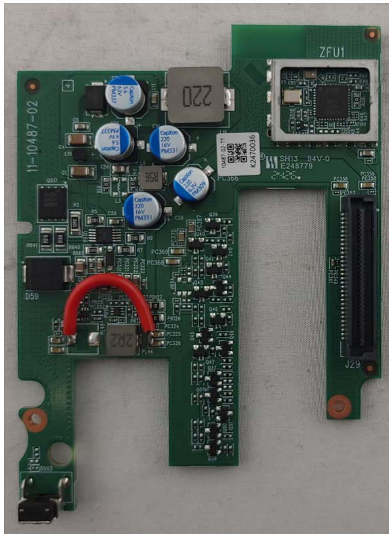
Photograph 5: Daughter Card Top without Can
