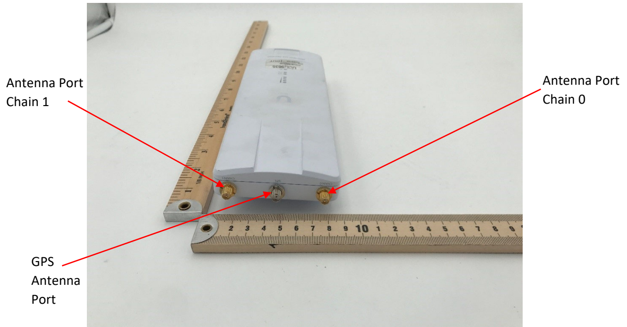
Photograph 5: Top View of DUT
