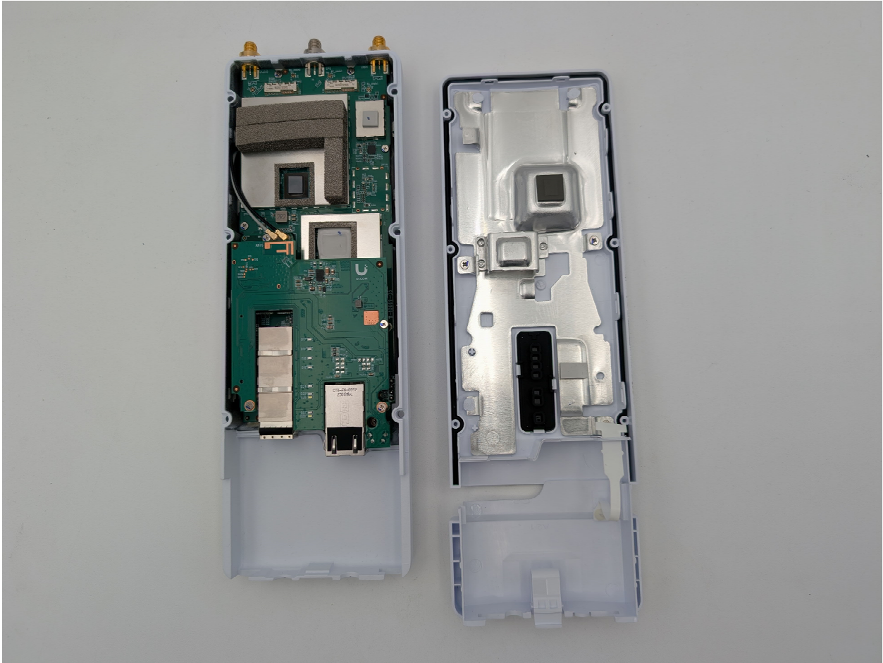
Photograph 1: Front Cover Off
