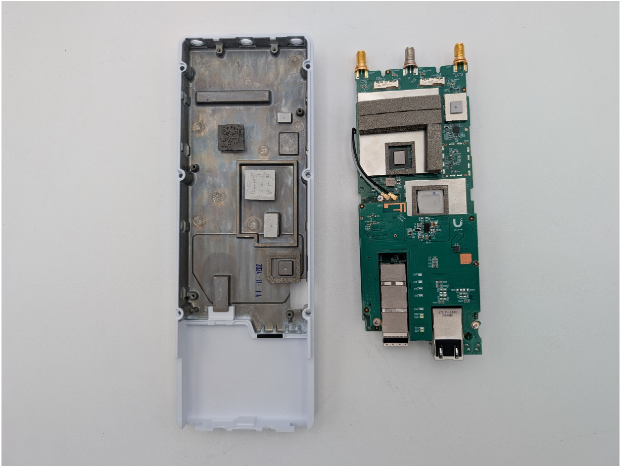
Photograph 1: PCB Out of Back Cover
