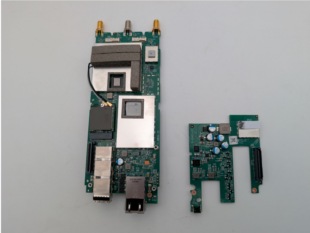
Photograph 1: Daughter PCB Removed
