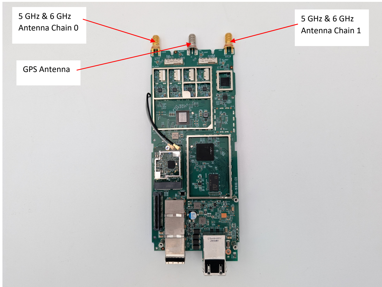
Photograph 2: Main PCB Top w/Cans Off
