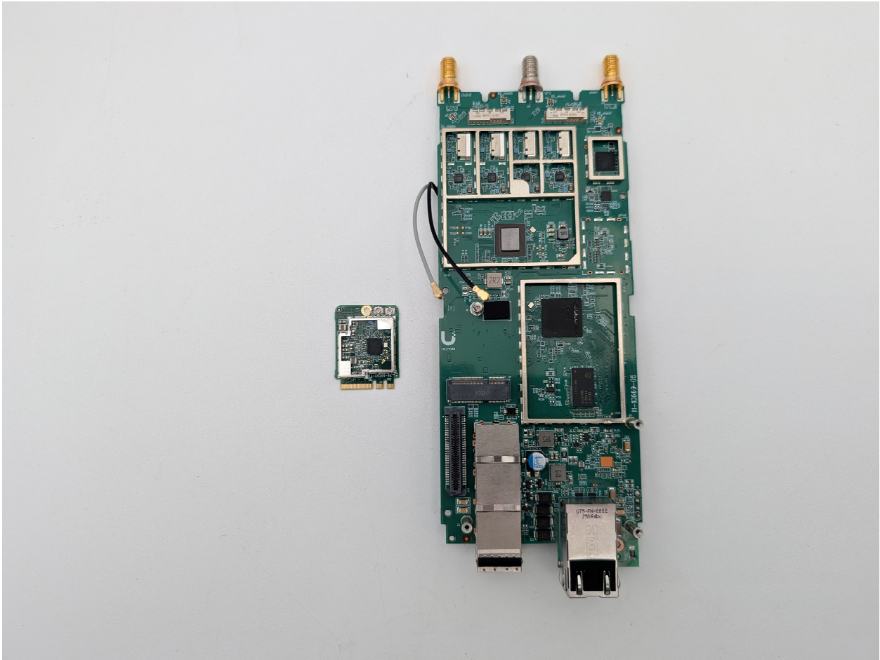
Photograph 2: GPS Scanner Radio Out of Main PCB
