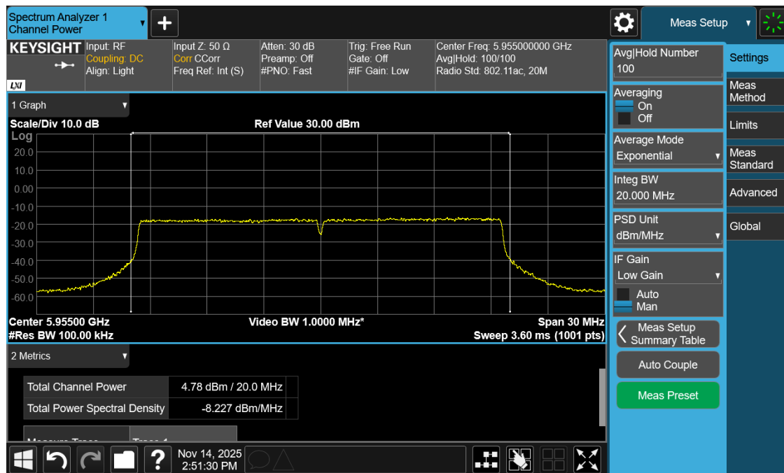
Plot 12: Power and PSD for Standard Power– 5955 MHz
