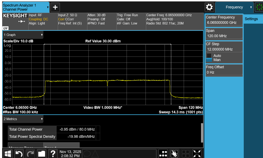
Plot 6: Power and PSD for Standard Power – 6065 MHz
