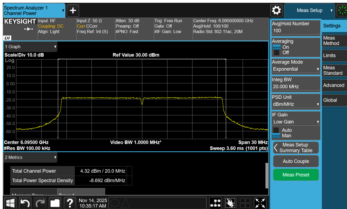
Plot 1: Power and PSD for Standard Power – 6095 MHz
