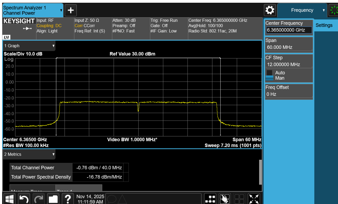
Plot 3: Power and PSD for Standard Power – 6365 MHz
