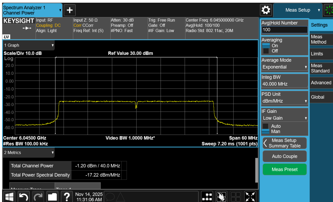
Plot 4: Power and PSD for Standard Power – 6045 MHz
