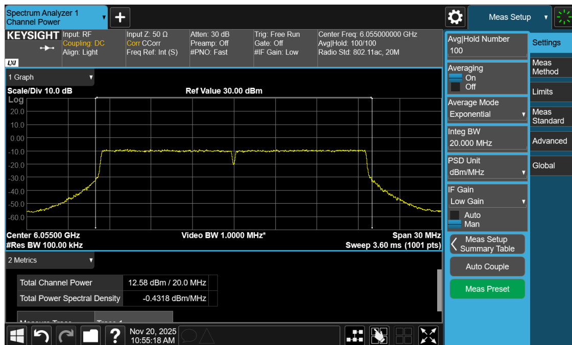
Plot 13: Power and PSD for Standard Power– 6055 MHz
