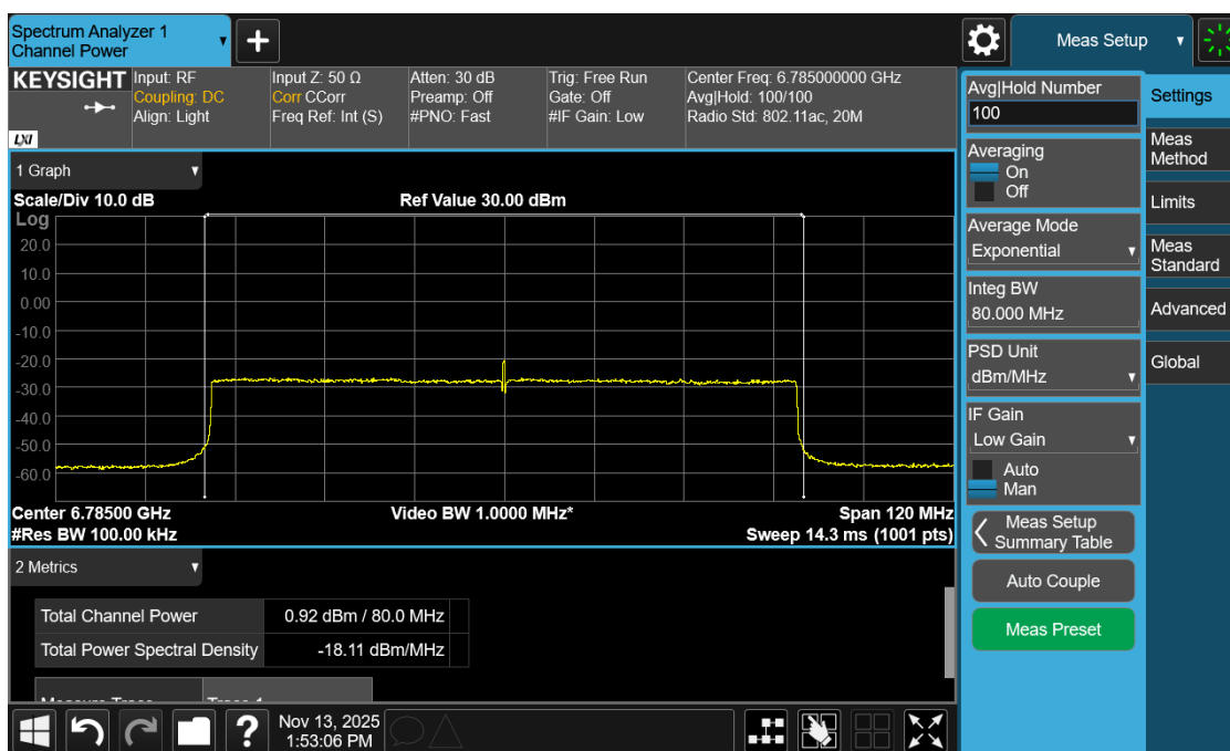
Plot 5: Power and PSD for Standard Power – 6785 MHz
