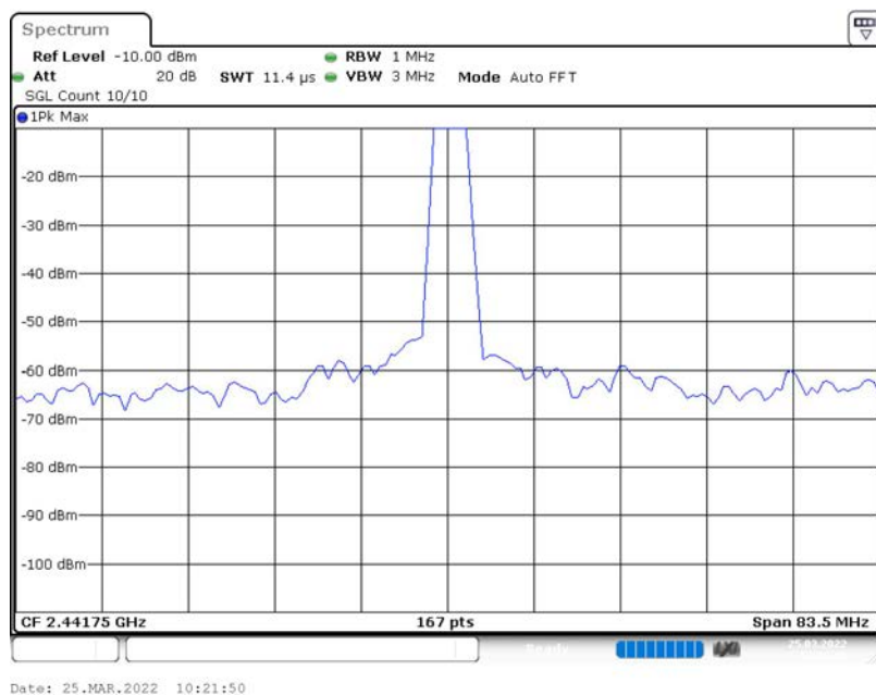
Restricted Band Connector 1_7
