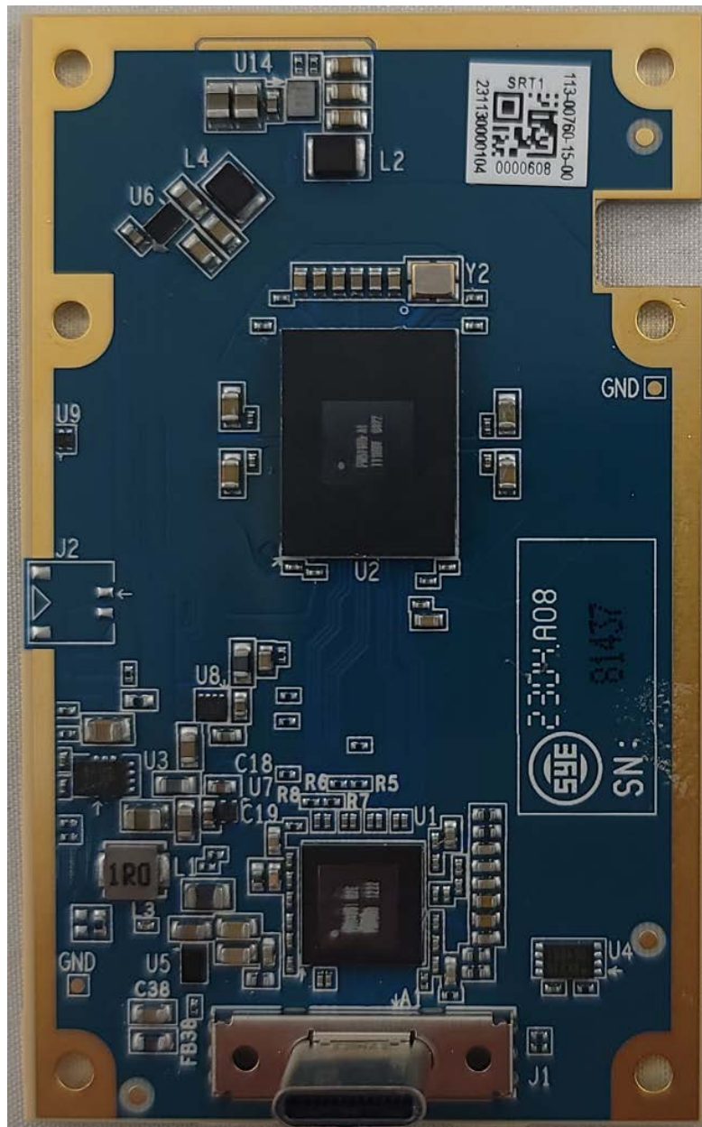
Photograph 4: Internal View of 60 GHz PCB Bottom
