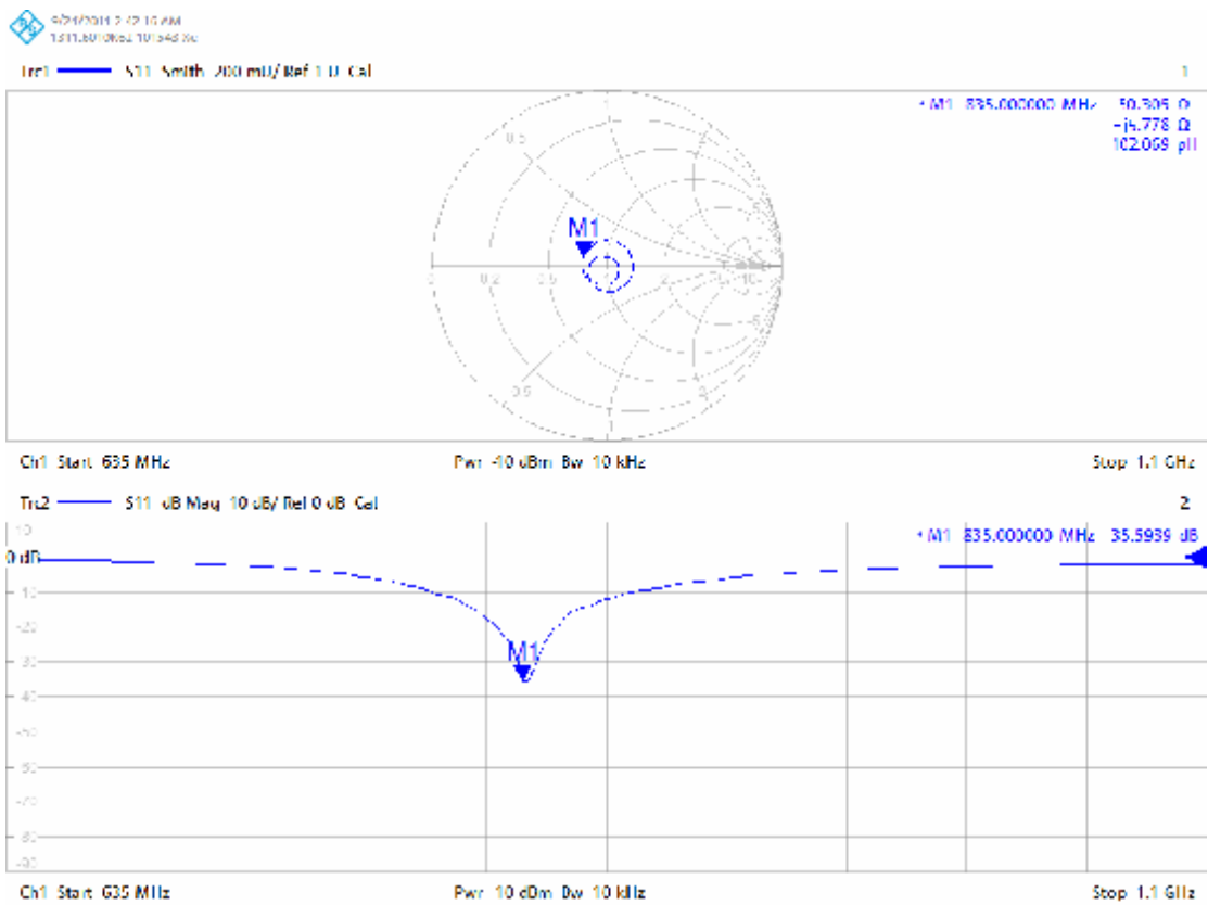
835MHz Dipole Body D835V2, serial No. 4d141 Extended Dipole Calibrations
