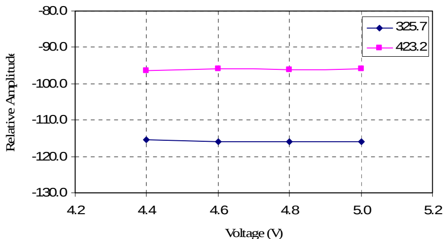
Figure 6.2. Relative emission at vs. supply voltage.
