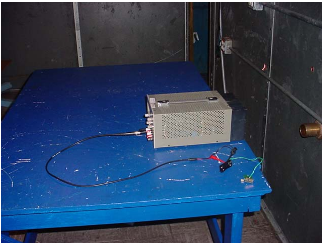
Conducted Emissions - Side
