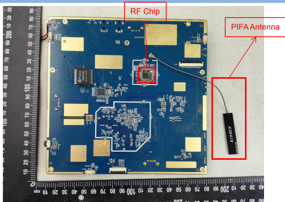
MAIN BOARD TOP VIEW 4
