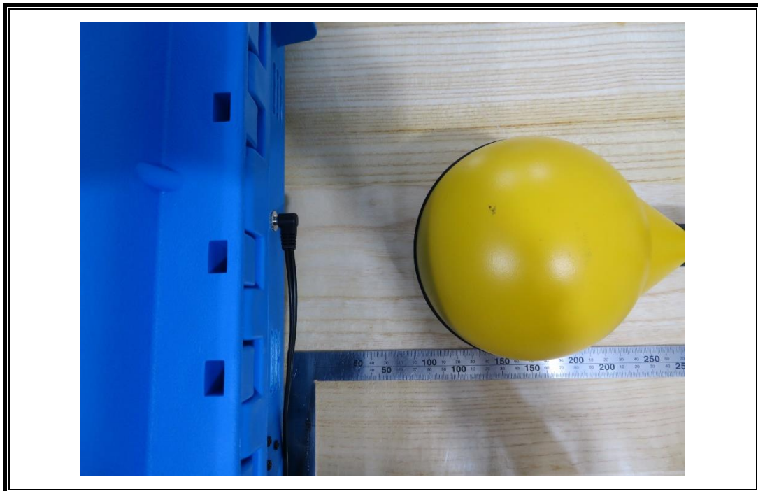
H-FILED STRENGTH MEASUREMENT SETUP FOR B POINT
