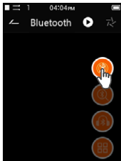
1. Enable Bluetooth.
