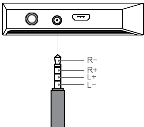
Pin Arrangement of Balanced Audio Port
