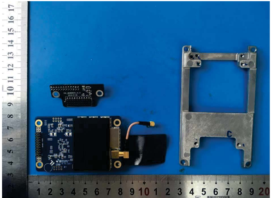
EUT View
