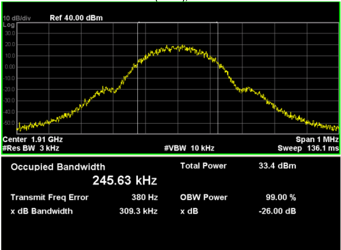
GPRS 1900 (8 Link), Channel 810
