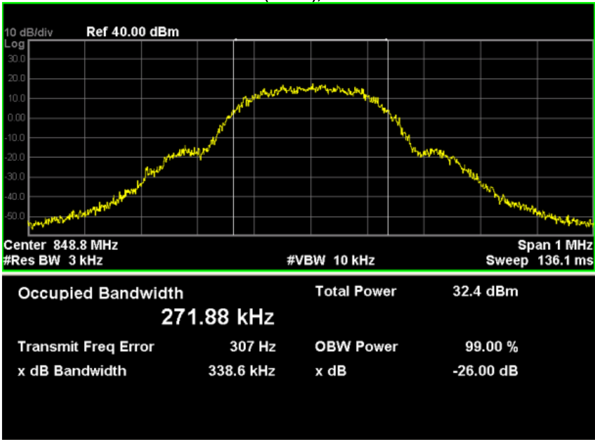
GPRS850 (8 Link), Channel 251
