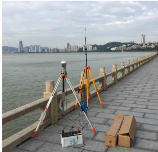
Figure 2-3 Set RTK Base Station
