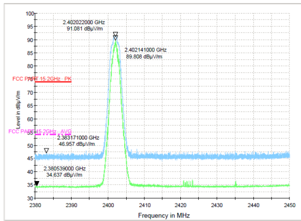
Test Mode: \pi/4 DQPSK-Low Hopping-off
