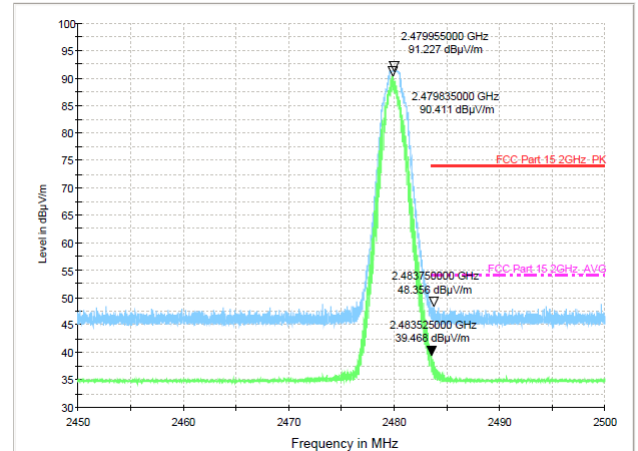
Test Mode: GFSK-High Hopping-off
