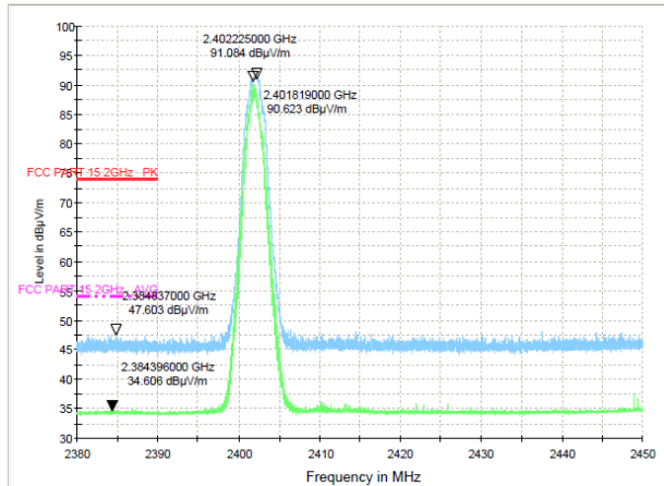
Test Mode: GFSK-Low Hopping-off
