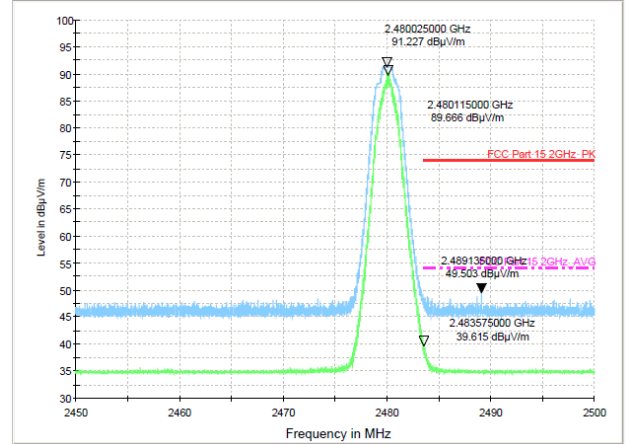
Test Mode: \pi/4 DQPSK-High Hopping-off
