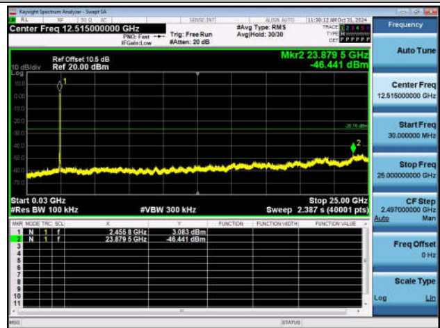
11N20SISO-Ant1-2462-30~25000-PASS
