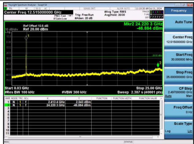
11N20SISO-Ant1-2437-30~25000-PASS
