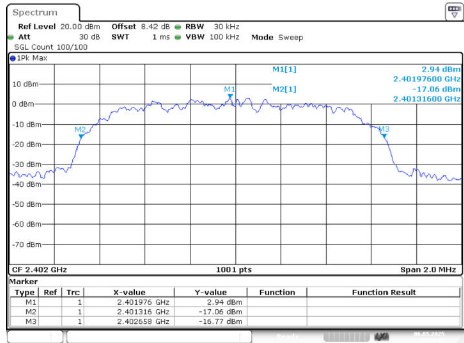
-20dB Bandwidth NVNT 2-DH5 2402MHz Ant1
