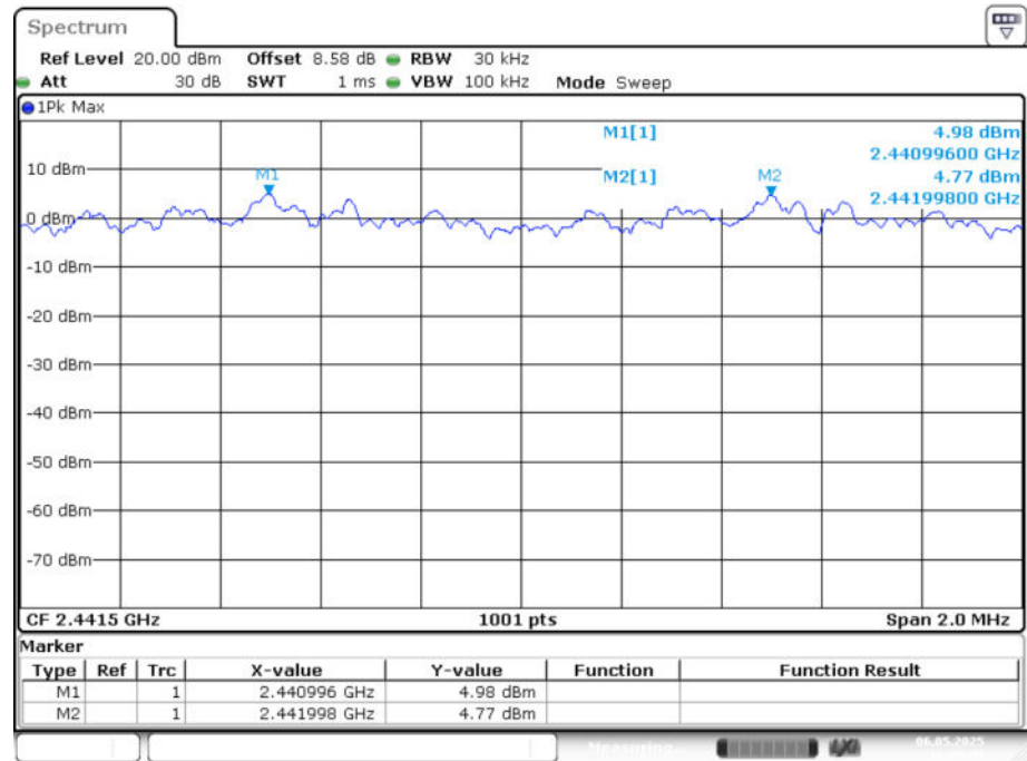
CFS NVNT 2-DH5 2441MHz Ant1
