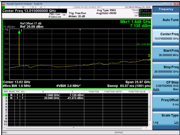
Test Mode: LTE Band 25 / 5MHz /25RB
