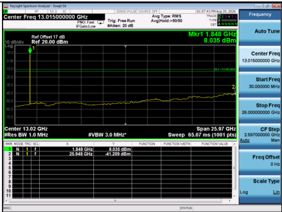
Test Mode: LTE Band 25 / 5MHz /1RB
