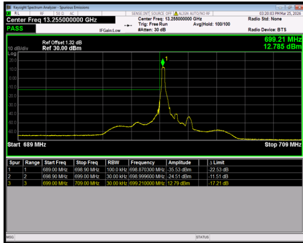
Band12 16QAM BW=1.4MHz LowChannel=23017 RB Size=1 Position=#0
