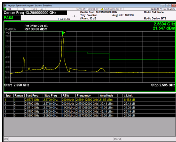
Band7 QPSK BW=10MHz HighChannel=21400 RB Size=1 Position=#Max
