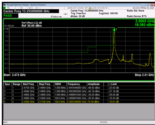
Band7 QPSK BW=5MHz LowChannel=20775 RB Size=1 Position=#0
