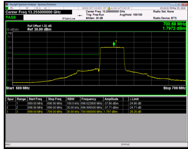
Band12 QPSK BW=3MHz LowChannel=23025 RB Size=15 Position=#0
