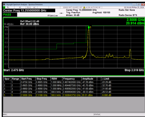
Band7 16QAM BW=15MHz LowChannel=20825 RB Size=1 Position=#0
