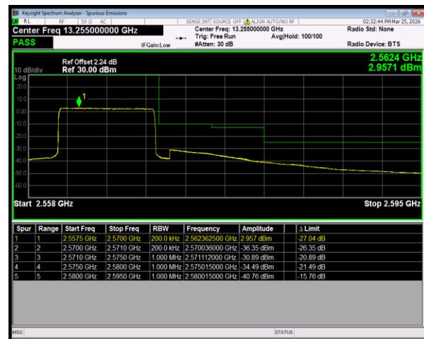
Band7 16QAM BW=10MHz HighChannel=21400 RB Size=50 Position=#0
