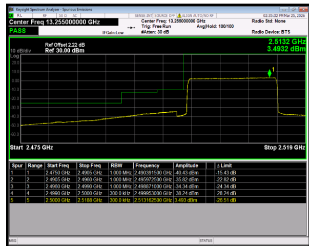
Band7 16QAM BW=15MHz LowChannel=20825 RB Size=75 Position=#0
