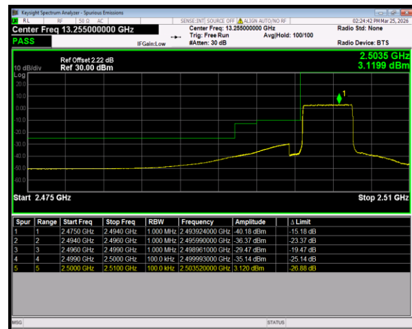
Band7 16QAM BW=5MHz LowChannel=20775 RB Size=25 Position=#0
