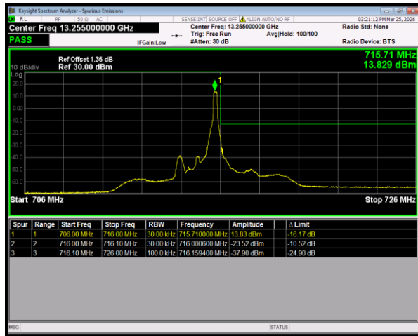
Band12 QPSK BW=1.4MHz HighChannel=23173 RB Size=1 Position=#Max
