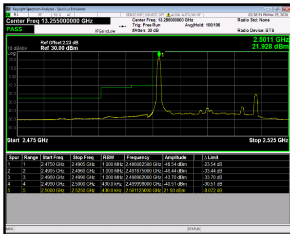
Band7 QPSK BW=20MHz LowChannel=20850 RB Size=1 Position=#0
