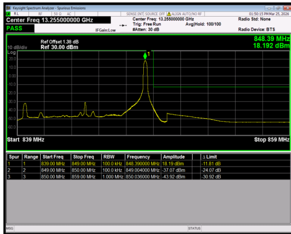
Band5 16QAM BW=10MHz HighChannel=20600 RB Size=1 Position=#Max
