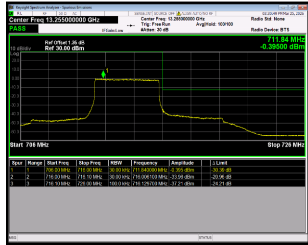
Band12 QPSK BW=5MHz HighChannel=23155 RB Size=25 Position=#0
