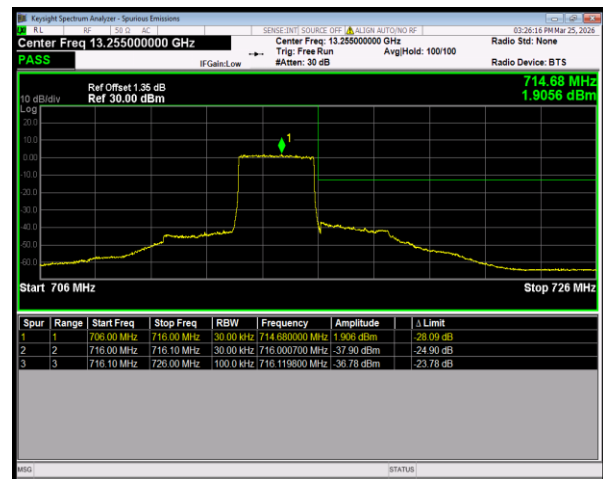
Band12 QPSK BW=3MHz HighChannel=23165 RB Size=15 Position=#0
