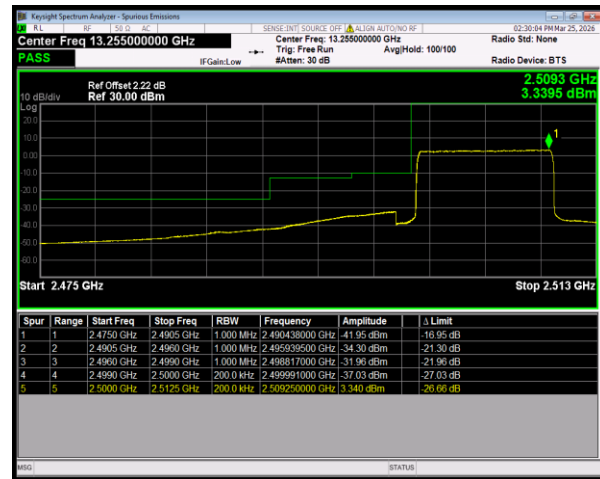
Band7 16QAM BW=10MHz LowChannel=20800 RB Size=50 Position=#0
