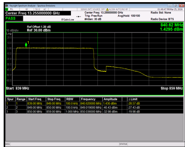
Band5 QPSK BW=10MHz HighChannel=20600 RB Size=50 Position=#0
