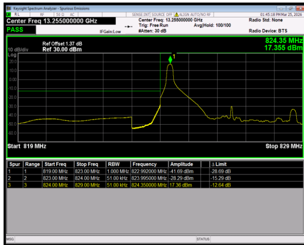
Band5 16QAM BW=5MHz LowChannel=20425 RB Size=1 Position=#0
