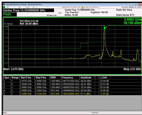
Band7 16QAM BW=5MHz LowChannel=20775 RB Size=1 Position=#0
