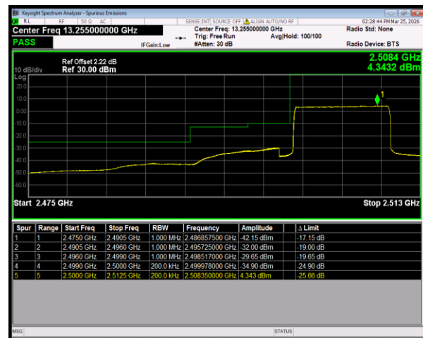
Band7 QPSK BW=10MHz LowChannel=20800 RB Size=50 Position=#0
