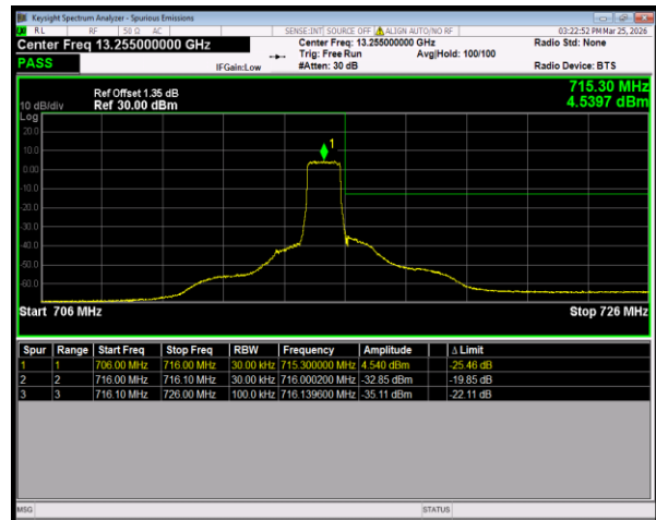
Band12 16QAM BW=1.4MHz HighChannel=23173 RB Size=6 Position=#0
