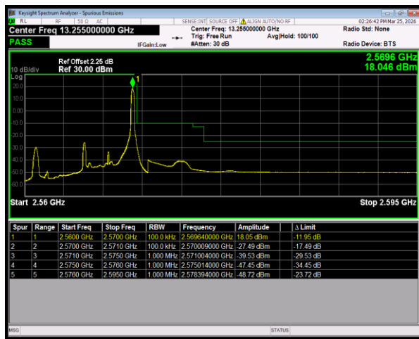
Band7 16QAM BW=5MHz HighChannel=21425 RB Size=1 Position=#Max
