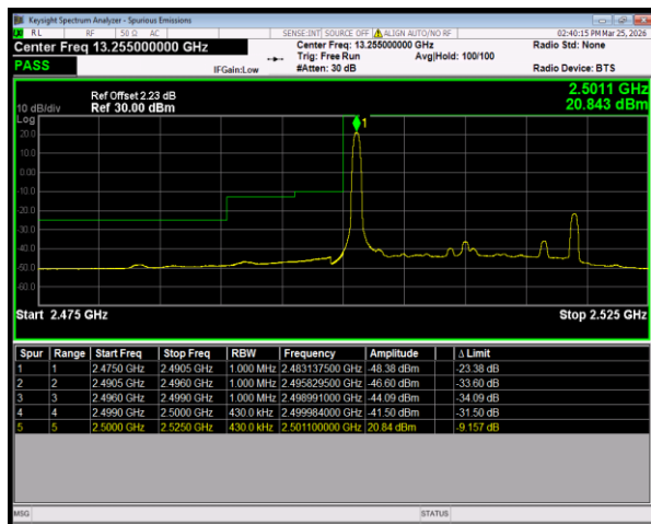
Band7 16QAM BW=20MHz LowChannel=20850 RB Size=1 Position=#0
