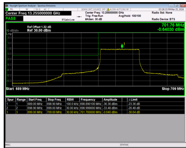
Band12 QPSK BW=5MHz LowChannel=23035 RB Size=25 Position=#0
