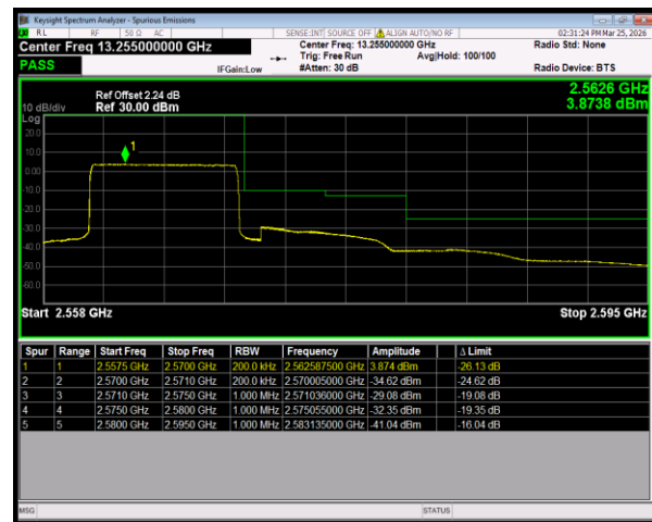
Band7 QPSK BW=10MHz HighChannel=21400 RB Size=50 Position=#0
