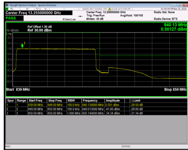
Band5 16QAM BW=10MHz HighChannel=20600 RB Size=50 Position=#0
