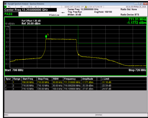
Band12 16QAM BW=5MHz HighChannel=23155 RB Size=25 Position=#0
