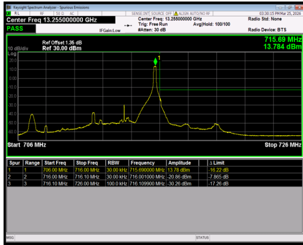
Band12 QPSK BW=5MHz HighChannel=23155 RB Size=1 Position=#Max
