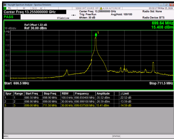
Band12 QPSK BW=10MHz LowChannel=23060 RB Size=1 Position=#0
