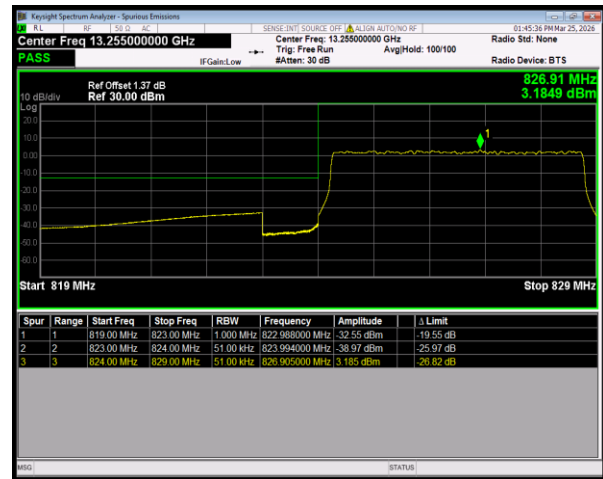
Band5 16QAM BW=5MHz LowChannel=20425 RB Size=25 Position=#0
