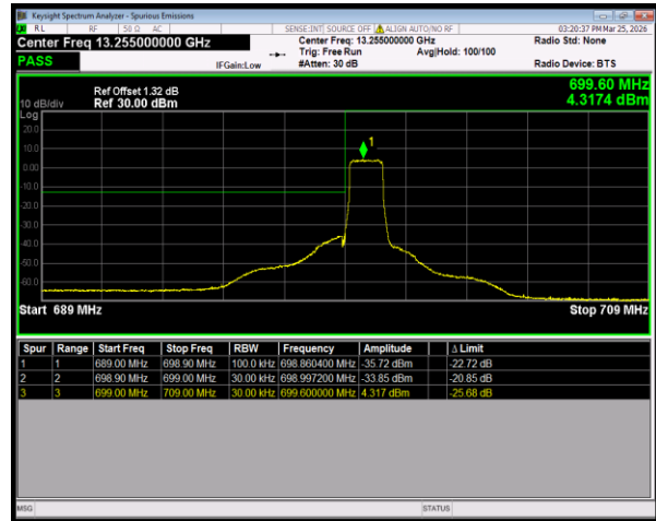
Band12 16QAM BW=1.4MHz LowChannel=23017 RB Size=6 Position=#0
