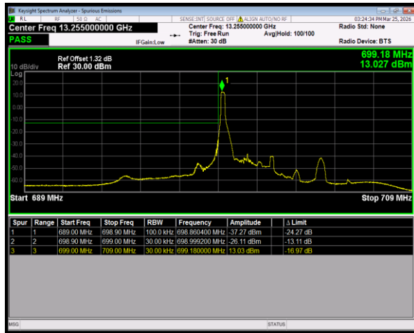
Band12 16QAM BW=3MHz LowChannel=23025 RB Size=1 Position=#0
