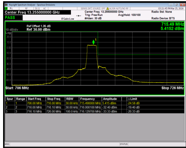
Band12 QPSK BW=1.4MHz HighChannel=23173 RB Size=6 Position=#0
