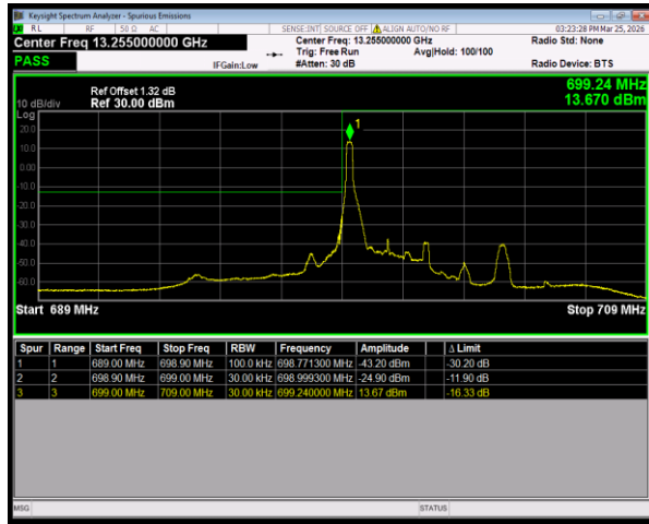
Band12 QPSK BW=3MHz LowChannel=23025 RB Size=1 Position=#0
