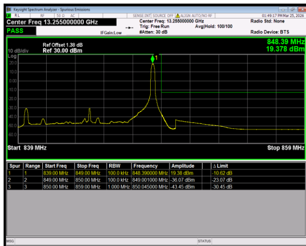
Band5 QPSK BW=10MHz HighChannel=20600 RB Size=1 Position=#Max
