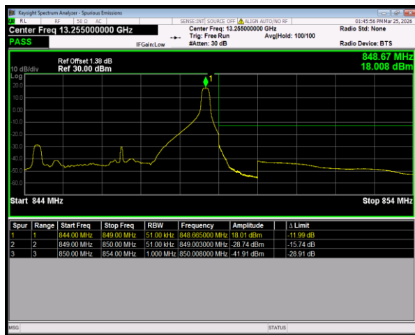
Band5 QPSK BW=5MHz HighChannel=20625 RB Size=1 Position=#Max
