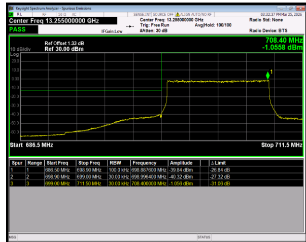
Band12 QPSK BW=10MHz LowChannel=23060 RB Size=50 Position=#0
