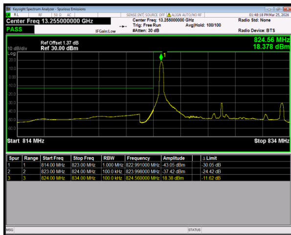
Band5 16QAM BW=10MHz LowChannel=20450 RB Size=1 Position=#0
