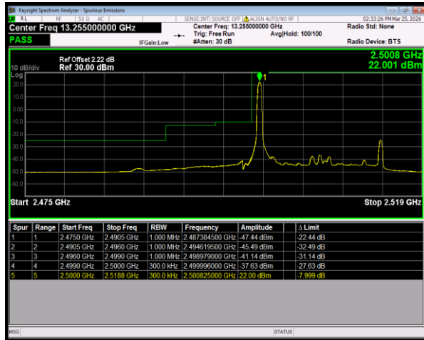
Band7 QPSK BW=15MHz LowChannel=20825 RB Size=1 Position=#0
