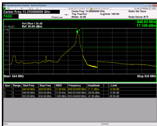
Band5 16QAM BW=5MHz HighChannel=20625 RB Size=1 Position=#Max
