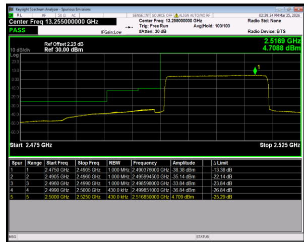
Band7 QPSK BW=20MHz LowChannel=20850 RB Size=100 Position=#0
