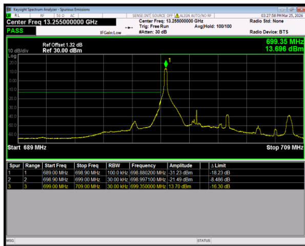
Band12 QPSK BW=5MHz LowChannel=23035 RB Size=1 Position=#0
