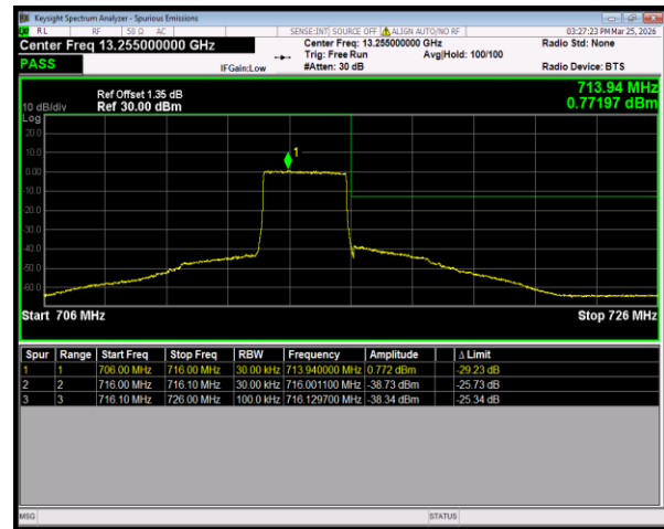
Band12 16QAM BW=3MHz HighChannel=23165 RB Size=15 Position=#0
