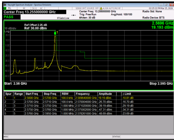
Band7 QPSK BW=5MHz HighChannel=21425 RB Size=1 Position=#Max
