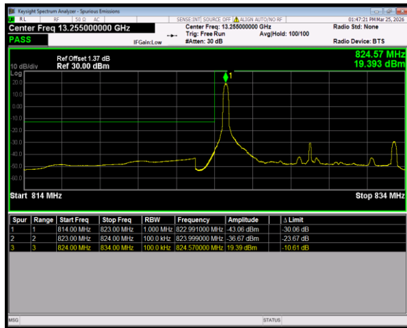
Band5 QPSK BW=10MHz LowChannel=20450 RB Size=1 Position=#0
