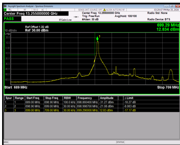
Band12 16QAM BW=5MHz LowChannel=23035 RB Size=1 Position=#0
