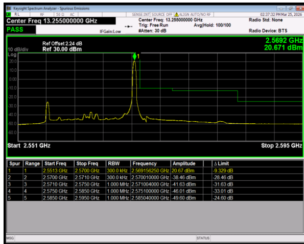
Band7 16QAM BW=15MHz HighChannel=21375 RB Size=1 Position=#Max
