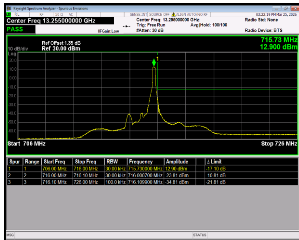
Band12 16QAM BW=1.4MHz HighChannel=23173 RB Size=1 Position=#Max
