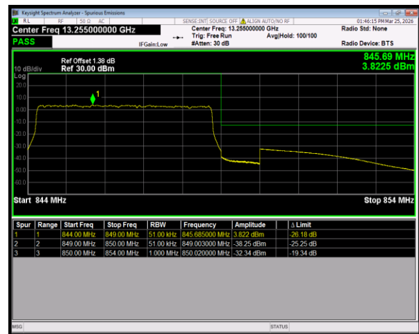
Band5 QPSK BW=5MHz HighChannel=20625 RB Size=25 Position=#0
