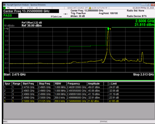
Band7 QPSK BW=10MHz LowChannel=20800 RB Size=1 Position=#0
