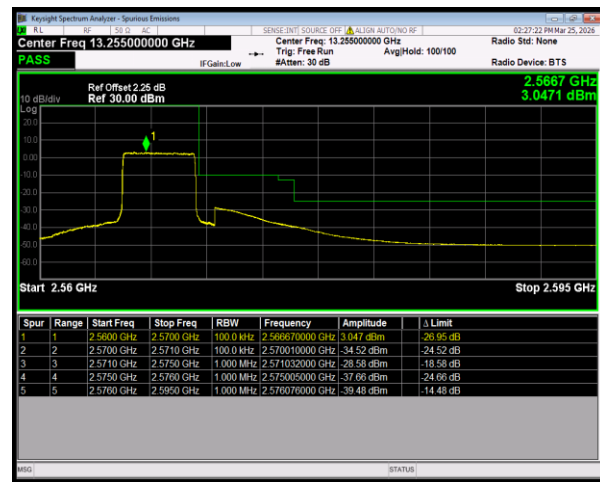
Band7 16QAM BW=5MHz HighChannel=21425 RB Size=25 Position=#0
