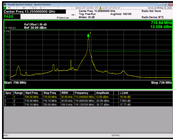
Band12 16QAM BW=5MHz HighChannel=23155 RB Size=1 Position=#Max
