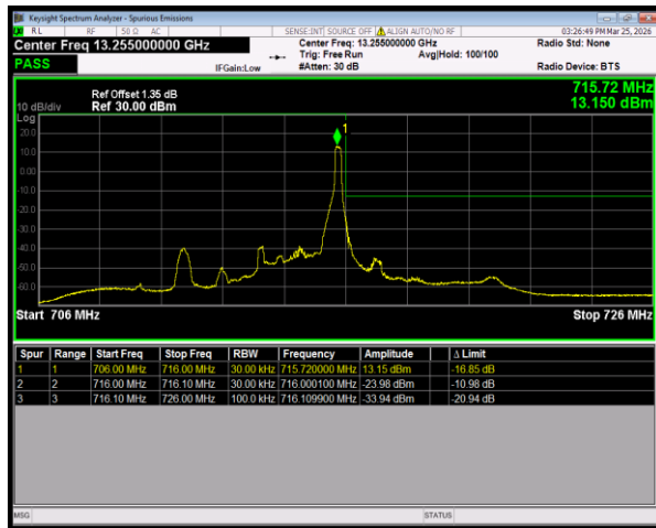
Band12 16QAM BW=3MHz HighChannel=23165 RB Size=1 Position=#Max
