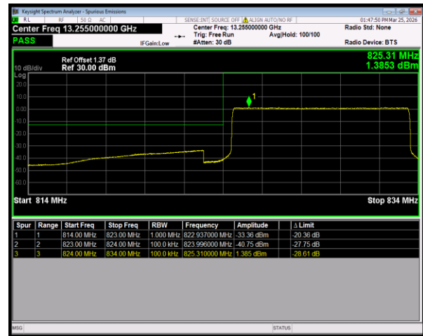
Band5 QPSK BW=10MHz LowChannel=20450 RB Size=50 Position=#0
