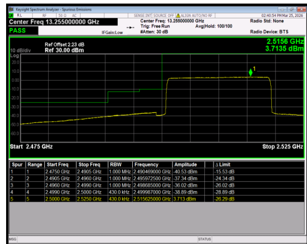
Band7 16QAM BW=20MHz LowChannel=20850 RB Size=100 Position=#0
