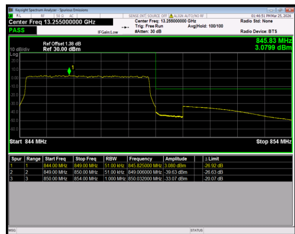
Band5 16QAM BW=5MHz HighChannel=20625 RB Size=25 Position=#0
