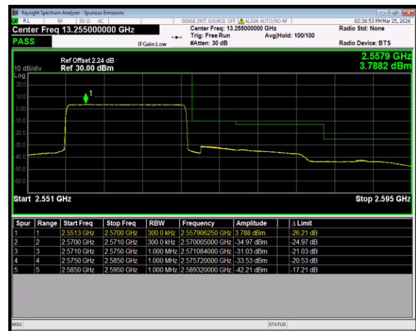
Band7 QPSK BW=15MHz HighChannel=21375 RB Size=75 Position=#0
