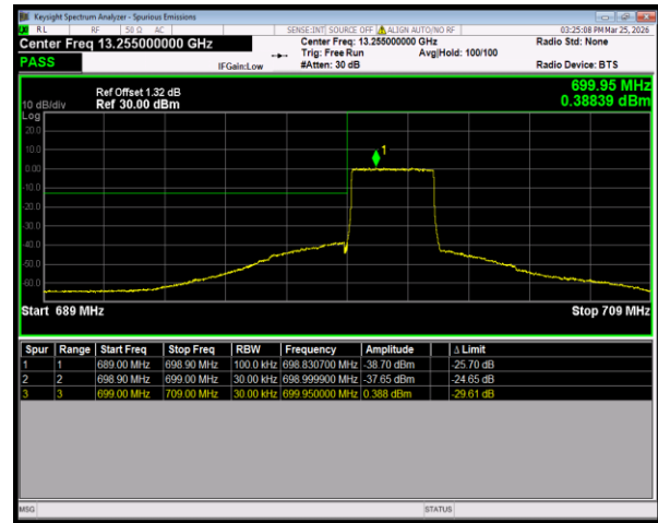
Band12 16QAM BW=3MHz LowChannel=23025 RB Size=15 Position=#0
