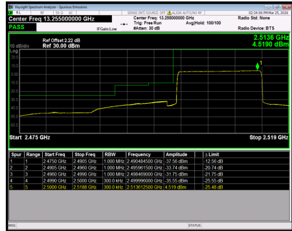
Band7 QPSK BW=15MHz LowChannel=20825 RB Size=75 Position=#0
