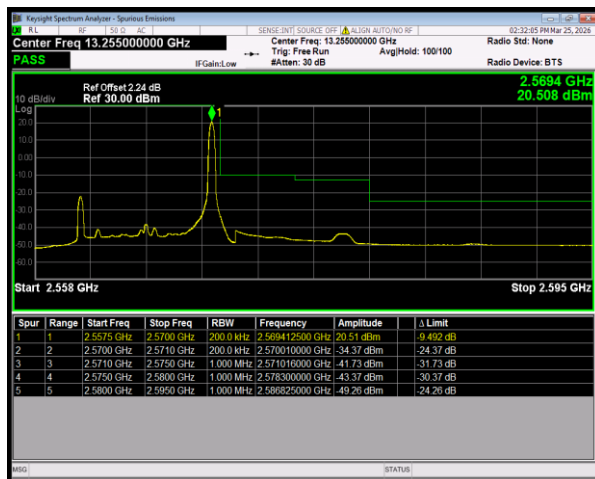
Band7 16QAM BW=10MHz HighChannel=21400 RB Size=1 Position=#Max
