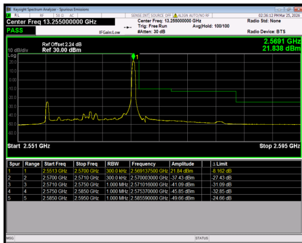
Band7 QPSK BW=15MHz HighChannel=21375 RB Size=1 Position=#Max
