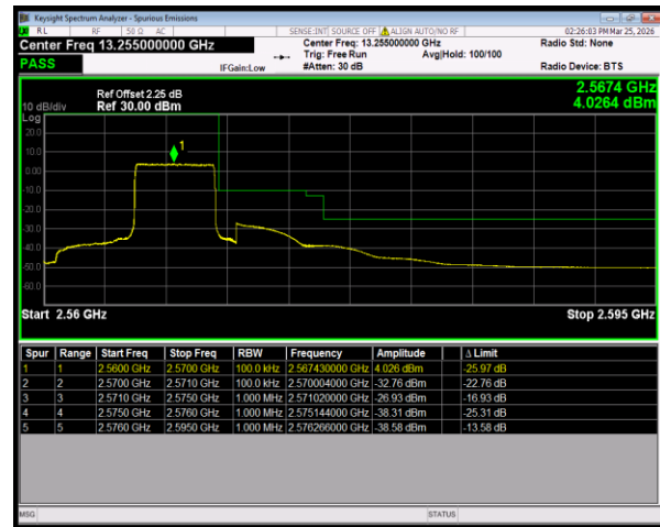
Band7 QPSK BW=5MHz HighChannel=21425 RB Size=25 Position=#0
