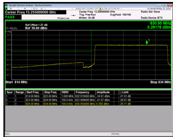
Band5 16QAM BW=10MHz LowChannel=20450 RB Size=50 Position=#0
