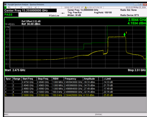
Band7 QPSK BW=5MHz LowChannel=20775 RB Size=25 Position=#0
