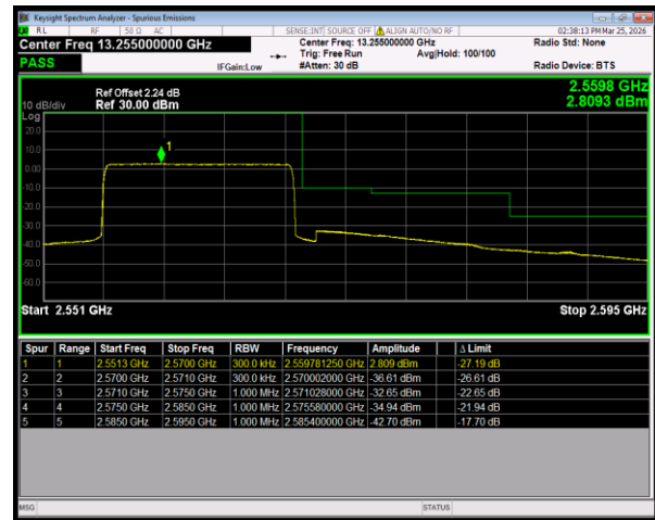
Band7 16QAM BW=15MHz HighChannel=21375 RB Size=75 Position=#0
