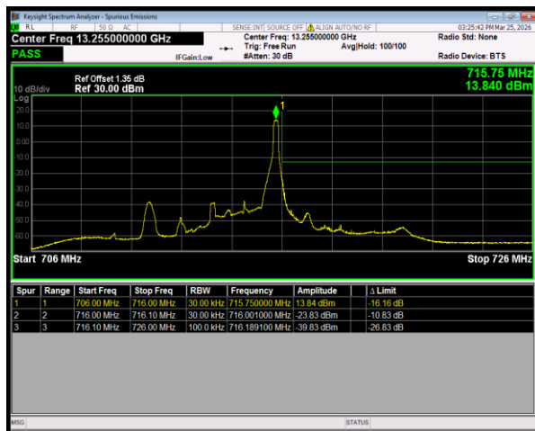
Band12 QPSK BW=3MHz HighChannel=23165 RB Size=1 Position=#Max
