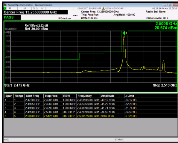
Band7 16QAM BW=10MHz LowChannel=20800 RB Size=1 Position=#0
