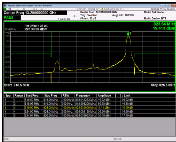
Band26(814-824) QPSK BW=5MHz HighChannel=26765 RB Size=1 Position=#Max
