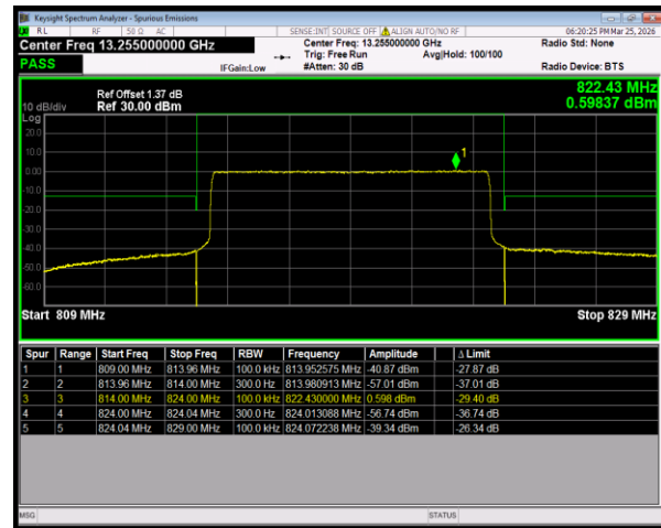
Band26(814-824) 16QAM BW=10MHz HighChannel=26740 RB Size=50 Position=#0
