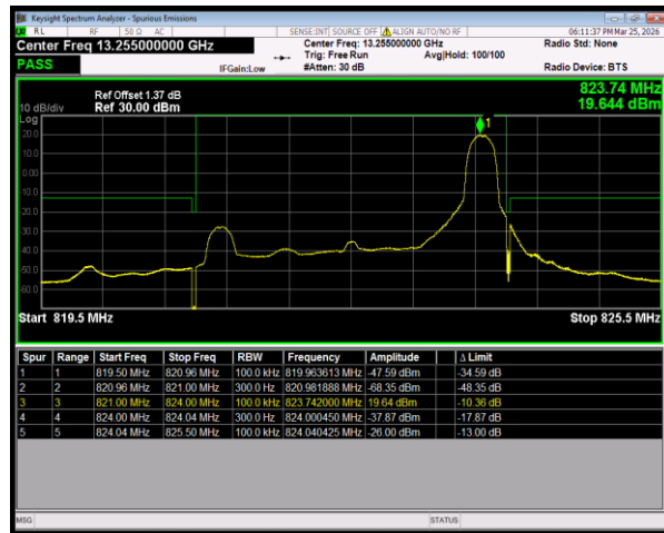
Band26(814-824) QPSK BW=3MHz HighChannel=26775 RB Size=1 Position=#Max
