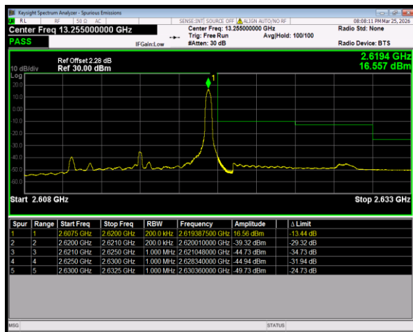
Band38 16QAM BW=10MHz HighChannel=38200 RB Size=1 Position=#Max
