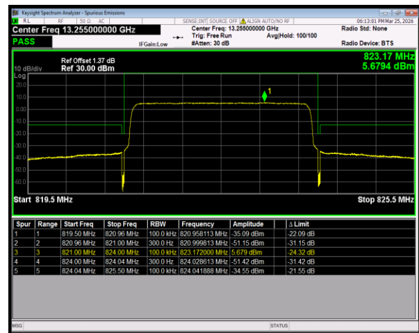
Band26(814-824) 16QAM BW=3MHz HighChannel=26775 RB Size=15 Position=#0
