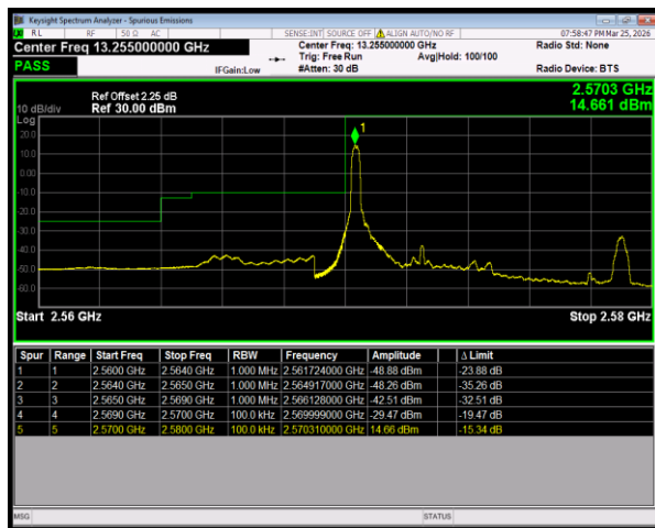
Band38 QPSK BW=5MHz LowChannel=37775 RB Size=1 Position=#0
