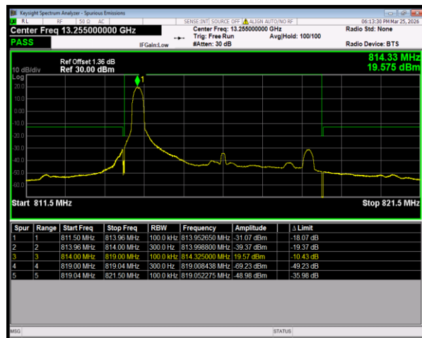
Band26(814-824) QPSK BW=5MHz LowChannel=26715 RB Size=1 Position=#0
