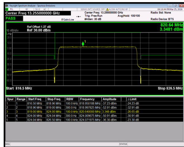
Band26(814-824) 16QAM BW=5MHz HighChannel=26765 RB Size=25 Position=#0
