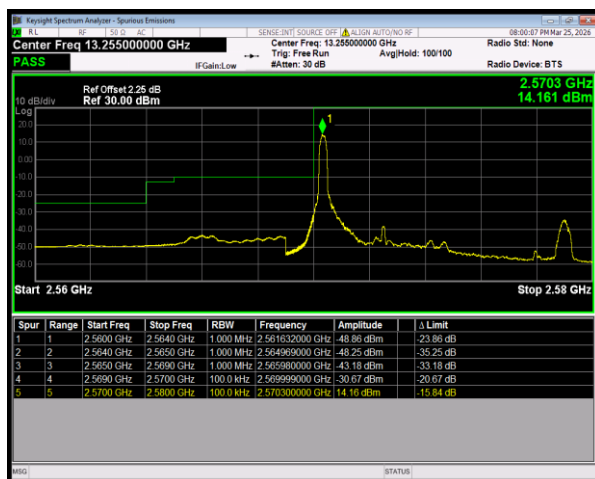
Band38 16QAM BW=5MHz LowChannel=37775 RB Size=1 Position=#0
