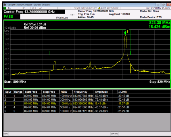
Band26(814-824) 16QAM BW=10MHz HighChannel=26740 RB Size=1 Position=#Max
