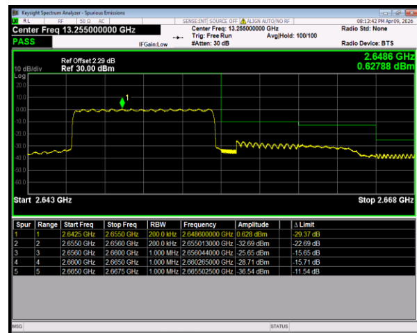
Band41(2535-2655) QPSK BW=10MHz HighChannel=41190 RB Size=50 Position=#0
