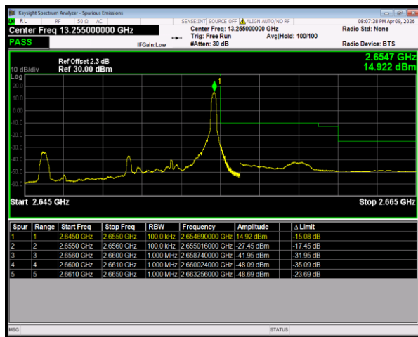
Band41(2535-2655) QPSK BW=5MHz HighChannel=41215 RB Size=1 Position=#Max
