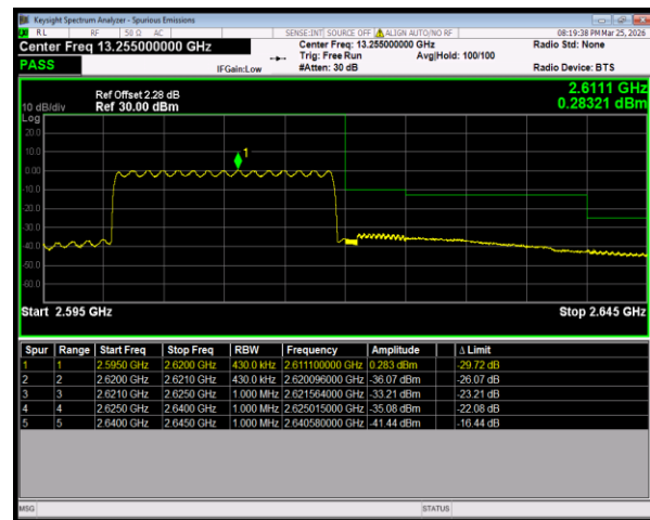
Band38 16QAM BW=20MHz HighChannel=38150 RB Size=100 Position=#0
