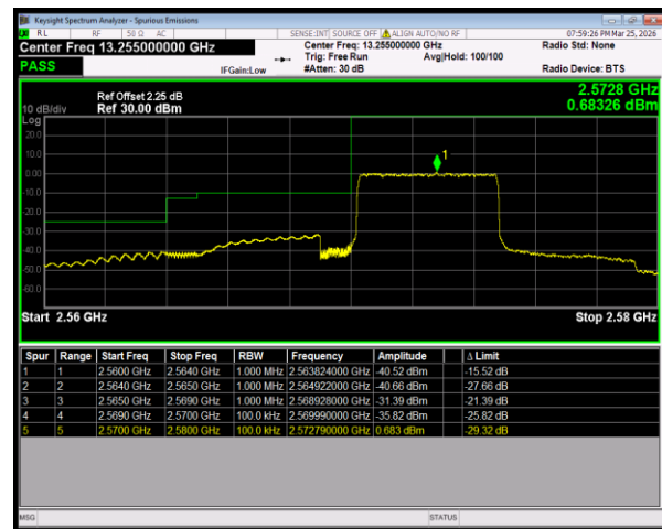
Band38 QPSK BW=5MHz LowChannel=37775 RB Size=25 Position=#0
