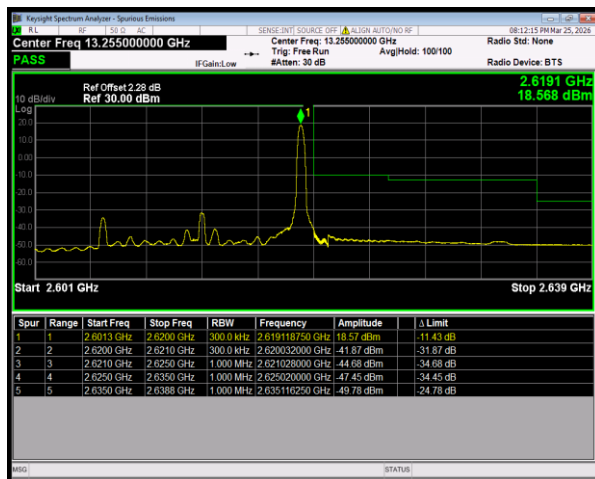
Band38 QPSK BW=15MHz HighChannel=38175 RB Size=1 Position=#Max
