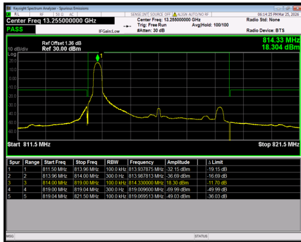
Band26(814-824) 16QAM BW=5MHz LowChannel=26715 RB Size=1 Position=#0
