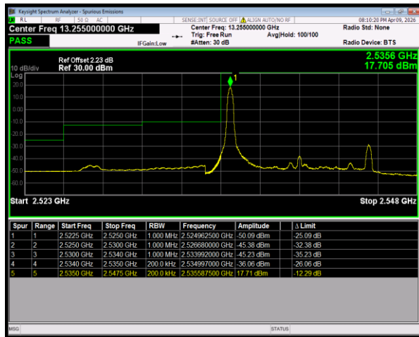
Band41(2535-2655) QPSK BW=10MHz LowChannel=40090 RB Size=1 Position=#0
