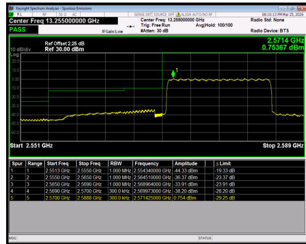
Band38 QPSK BW=15MHz LowChannel=37825 RB Size=75 Position=#0
