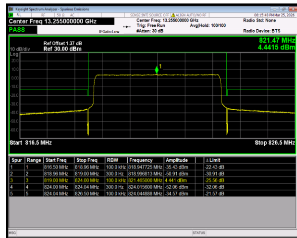
Band26(814-824) QPSK BW=5MHz HighChannel=26765 RB Size=25 Position=#0
