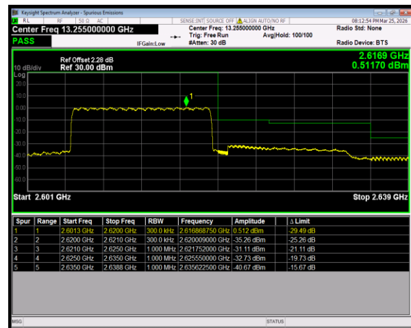
Band38 QPSK BW=15MHz HighChannel=38175 RB Size=75 Position=#0
