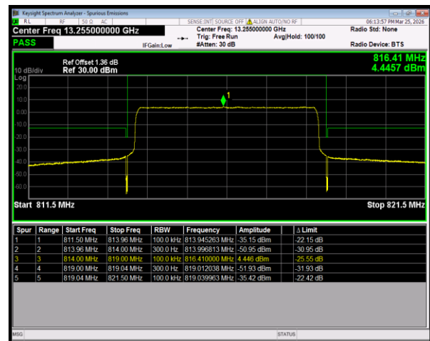
Band26(814-824) QPSK BW=5MHz LowChannel=26715 RB Size=25 Position=#0
