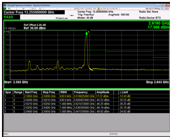
Band38 16QAM BW=20MHz HighChannel=38150 RB Size=1 Position=#Max
