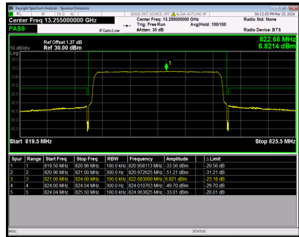
Band26(814-824) QPSK BW=3MHz HighChannel=26775 RB Size=15 Position=#0
