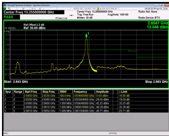
Band41(2535-2655) 16QAM BW=5MHz HighChannel=41215 RB Size=1 Position=#Max
