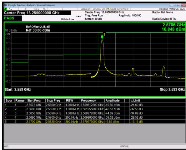
Band38 16QAM BW=10MHz LowChannel=37800 RB Size=1 Position=#0
