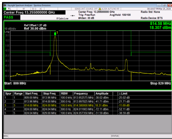
Band26(814-824) 16QAM BW=10MHz LowChannel=26740 RB Size=1 Position=#0
