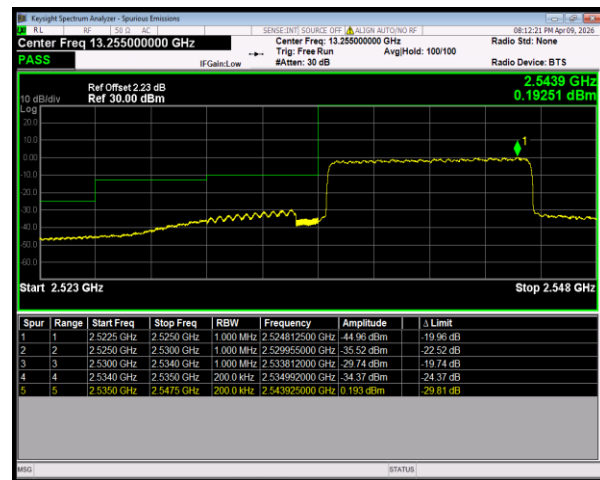
Band41(2535-2655) 16QAM BW=10MHz LowChannel=40090 RB Size=50 Position=#0
