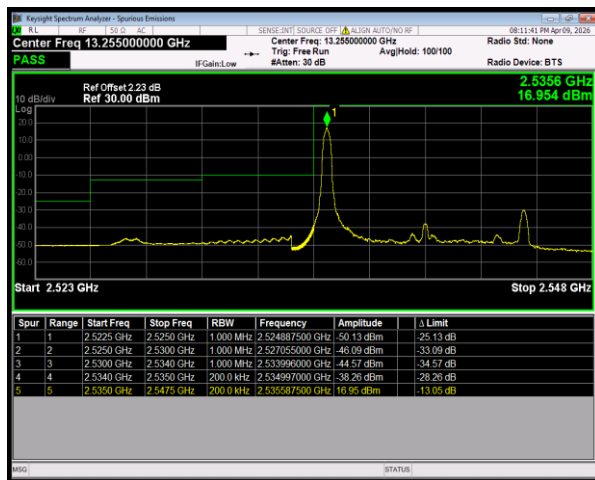
Band41(2535-2655) 16QAM BW=10MHz LowChannel=40090 RB Size=1 Position=#0
