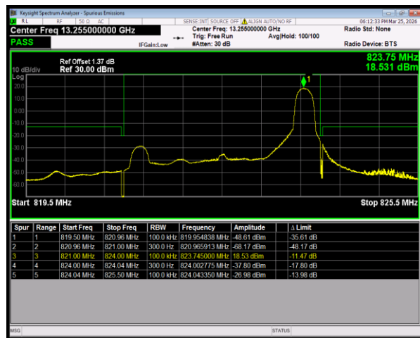
Band26(814-824) 16QAM BW=3MHz HighChannel=26775 RB Size=1 Position=#Max
