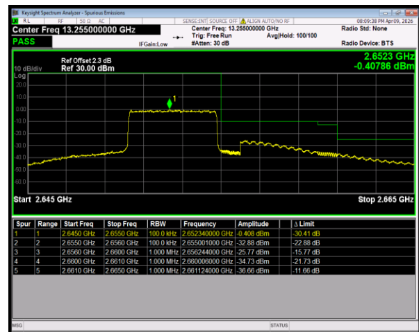
Band41(2535-2655) 16QAM BW=5MHz HighChannel=41215 RB Size=25 Position=#0
