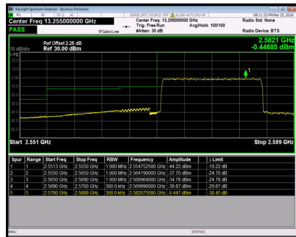
Band38 16QAM BW=15MHz LowChannel=37825 RB Size=75 Position=#0
