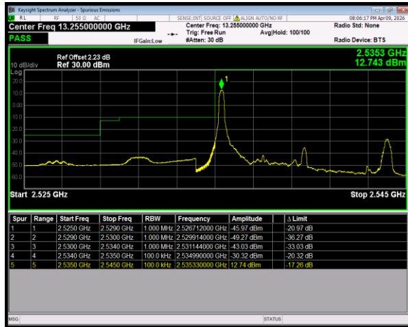
Band41(2535-2655) 16QAM BW=5MHz LowChannel=40065 RB Size=1 Position=#0
