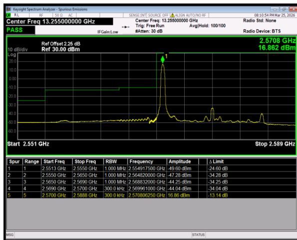
Band38 16QAM BW=15MHz LowChannel=37825 RB Size=1 Position=#0
