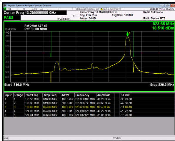
Band26(814-824) 16QAM BW=5MHz HighChannel=26765 RB Size=1 Position=#Max
