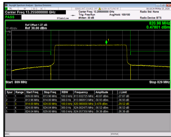
Band26(814-824) 16QAM BW=10MHz LowChannel=26740 RB Size=50 Position=#0
