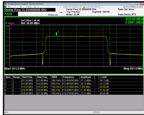
Band26(814-824) 16QAM BW=5MHz LowChannel=26715 RB Size=25 Position=#0
