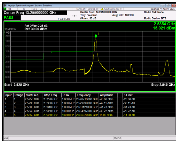
Band41(2535-2655) QPSK BW=5MHz LowChannel=40065 RB Size=1 Position=#0
