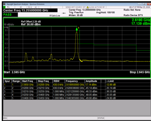
Band38 QPSK BW=20MHz HighChannel=38150 RB Size=1 Position=#Max
