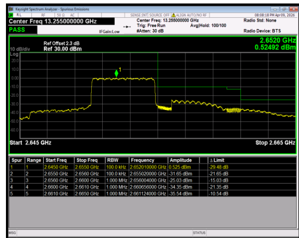
Band41(2535-2655) QPSK BW=5MHz HighChannel=41215 RB Size=25 Position=#0
