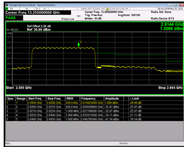
Band38 QPSK BW=20MHz HighChannel=38150 RB Size=100 Position=#0
