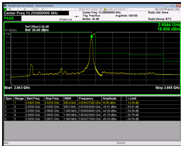
Band41(2535-2655) QPSK BW=10MHz HighChannel=41190 RB Size=1 Position=#Max
