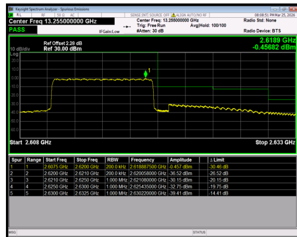
Band38 16QAM BW=10MHz HighChannel=38200 RB Size=50 Position=#0
