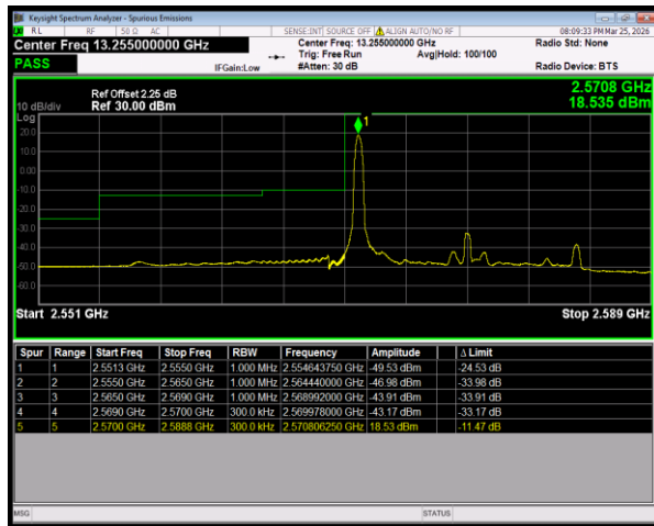
Band38 QPSK BW=15MHz LowChannel=37825 RB Size=1 Position=#0
