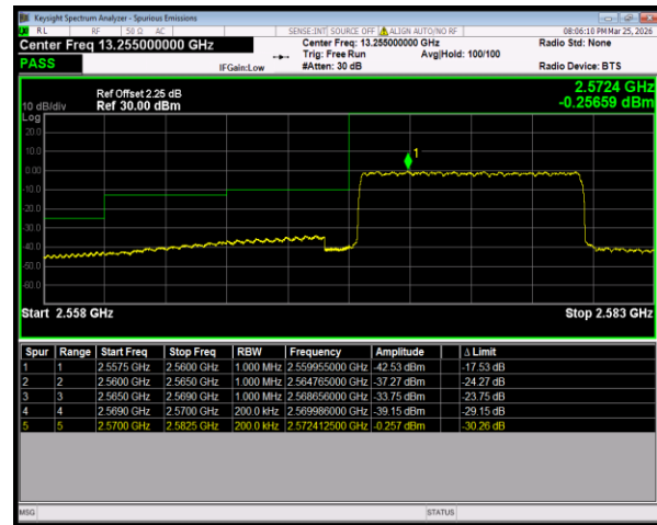
Band38 16QAM BW=10MHz LowChannel=37800 RB Size=50 Position=#0
