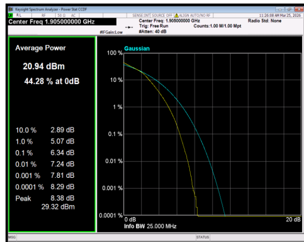
Band2 16QAM BW=10MHz Channel=19150 RB Size=50 Position=#0
