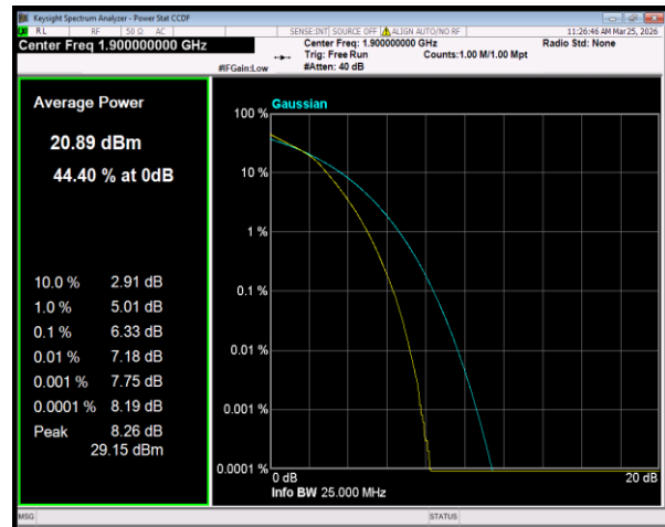
Band2 16QAM BW=20MHz Channel=19100 RB Size=100 Position=#0
