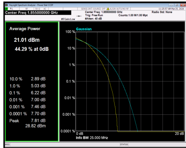
Band2 16QAM BW=10MHz Channel=18650 RB Size=50 Position=#0
