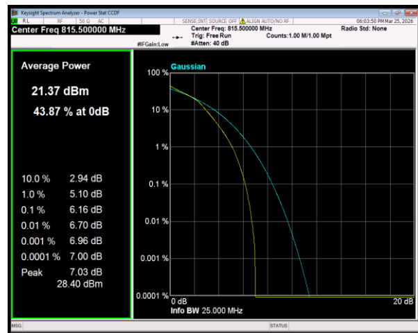
Band26(814-824) 16QAM BW=3MHz Channel=26705 RB Size=15 Position=#0
