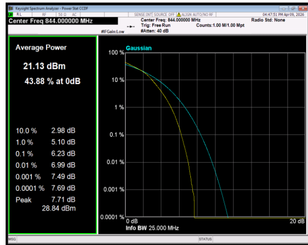
Band26(824-849) 16QAM BW=10MHz Channel=26990 RB Size=50 Position=#0
