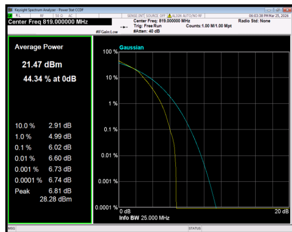
Band26(814-824) 16QAM BW=1.4MHz Channel=26740 RB Size=6 Position=#0
