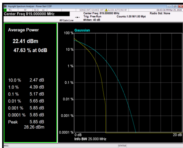
Band26(814-824) QPSK BW=1.4MHz Channel=26740 RB Size=6 Position=#0
