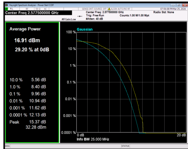
Band38 16QAM BW=15MHz Channel=37825 RB Size=75 Position=#0
