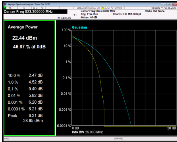
Band26(814-824) QPSK BW=1.4MHz Channel=26783 RB Size=6 Position=#0
