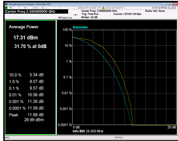
Band38 16QAM BW=10MHz Channel=38000 RB Size=50 Position=#0
