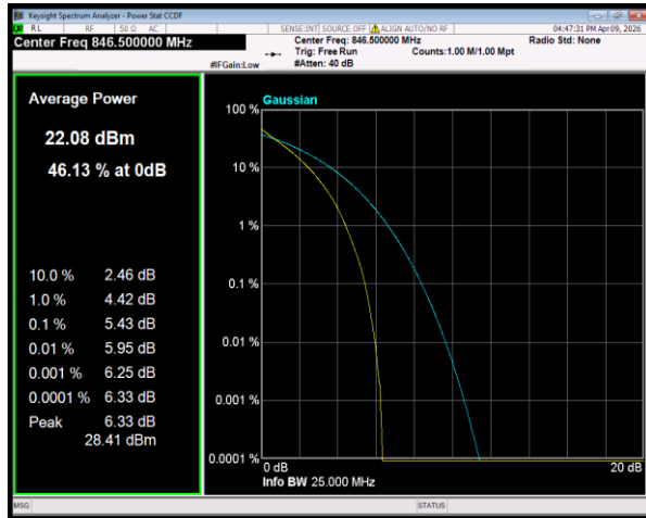
Band26(824-849) QPSK BW=5MHz Channel=27015 RB Size=25 Position=#0
