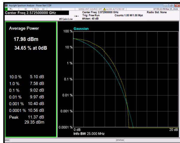
Band38 16QAM BW=5MHz Channel=37775 RB Size=25 Position=#0
