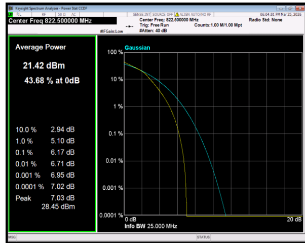
Band26(814-824) 16QAM BW=3MHz Channel=26775 RB Size=15 Position=#0
