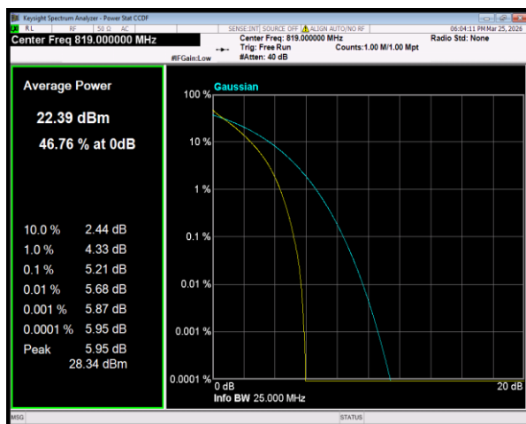
Band26(814-824) QPSK BW=5MHz Channel=26740 RB Size=25 Position=#0
