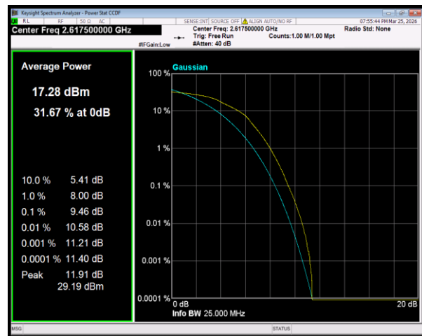
Band38 16QAM BW=5MHz Channel=38225 RB Size=25 Position=#0
