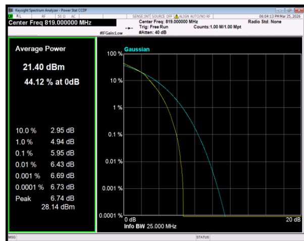
Band26(814-824) 16QAM BW=5MHz Channel=26740 RB Size=25 Position=#0
