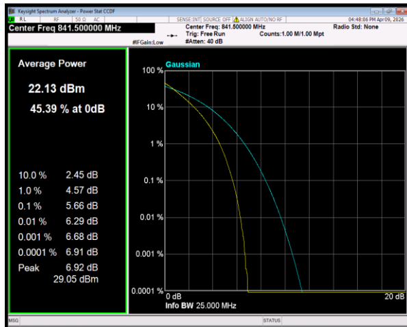
Band26(824-849) QPSK BW=15MHz Channel=26965 RB Size=75 Position=#0
