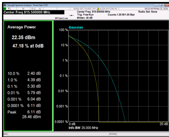
Band26(814-824) QPSK BW=3MHz Channel=26705 RB Size=15 Position=#0
