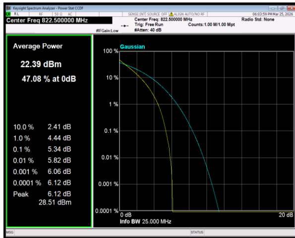
Band26(814-824) QPSK BW=3MHz Channel=26775 RB Size=15 Position=#0
