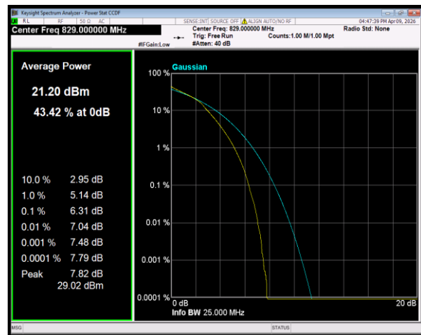
Band26(824-849) 16QAM BW=10MHz Channel=26840 RB Size=50 Position=#0
