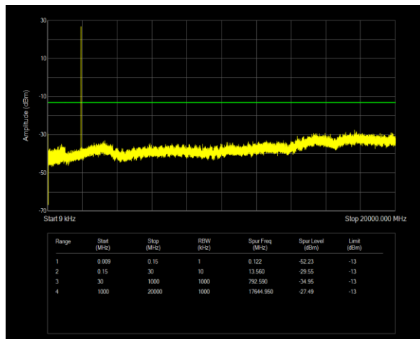
GPRS1900 Channel=810 NVNT
