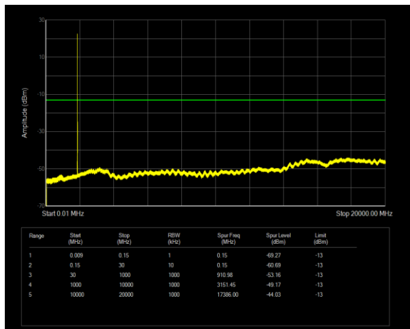
Band25 QPSK BW=5MHz Channel=26065 RB Size=1 Position=#0
