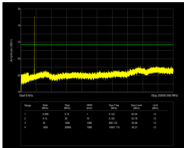
WCDMA Band4 Channel=1513 NVNT
