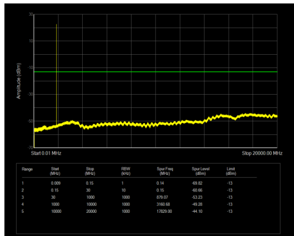
Band25 QPSK BW=1.4MHz Channel=26047 RB Size=1 Position=#0
