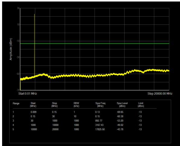
Band25 QPSK BW=1.4MHz Channel=26683 RB Size=1 Position=#0
