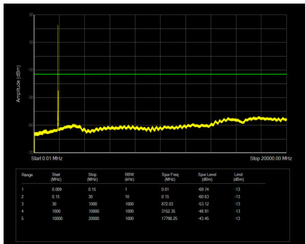
Band2 QPSK BW=20MHz Channel=18900 RB Size=1 Position=#0
