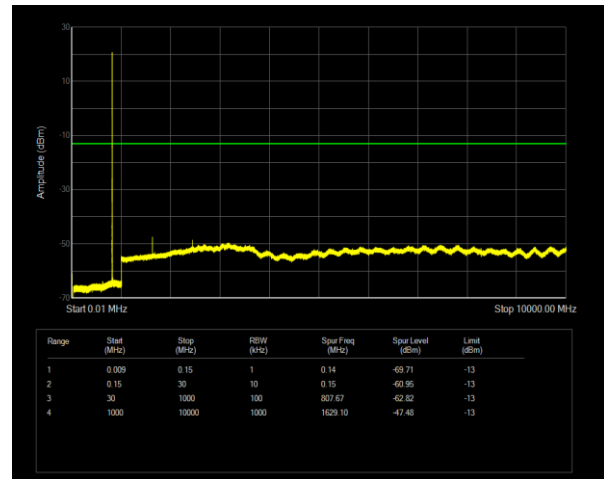
Band26(814-824) QPSK BW=1.4MHz Channel=26697 RB Size=1 Position=#0
