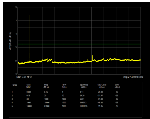
Band41(2535-2655) QPSK BW=5MHz Channel=41215 RB Size=1 Position=#0
