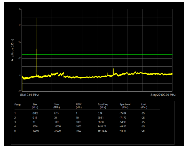
Band41(2535-2655) QPSK BW=15MHz Channel=40115 RB Size=1 Position=#0
