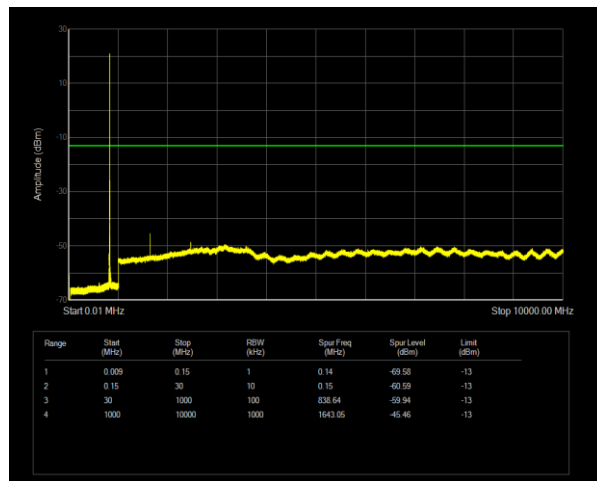
Band26(814-824) QPSK BW=3MHz Channel=26775 RB Size=1 Position=#0
