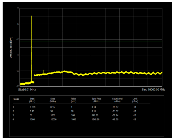
Band26(824-849) QPSK BW=1.4MHz Channel=26797 RB Size=1 Position=#0
