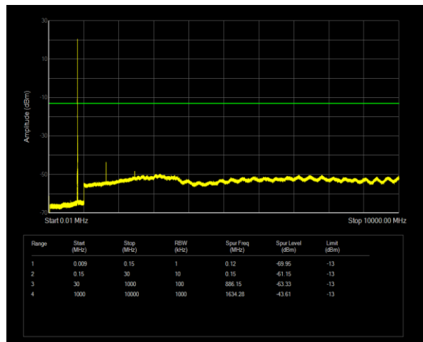
Band26(814-824) QPSK BW=5MHz Channel=26740 RB Size=1 Position=#0
