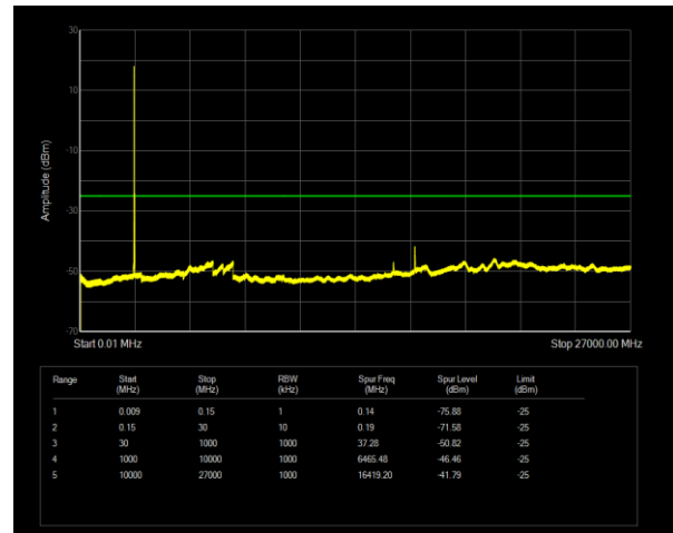
Band41(2535-2655) QPSK BW=15MHz Channel=41165 RB Size=1 Position=#0
