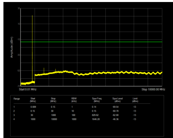
Band26(814-824) QPSK BW=1.4MHz Channel=26783 RB Size=1 Position=#0
