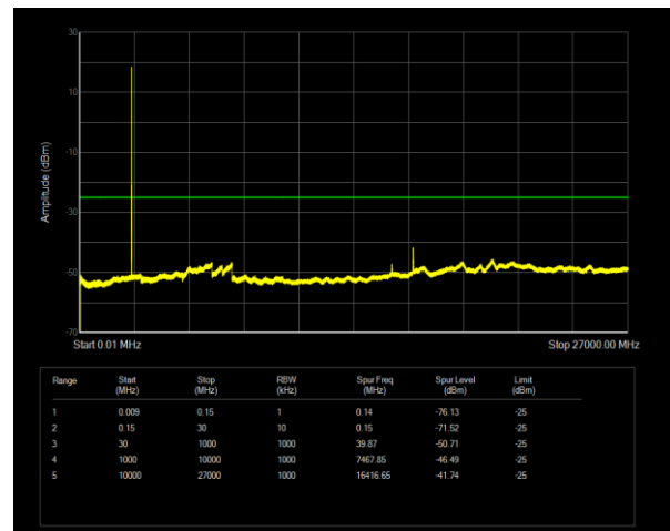
Band41(2535-2655) QPSK BW=5MHz Channel=40065 RB Size=1 Position=#0
