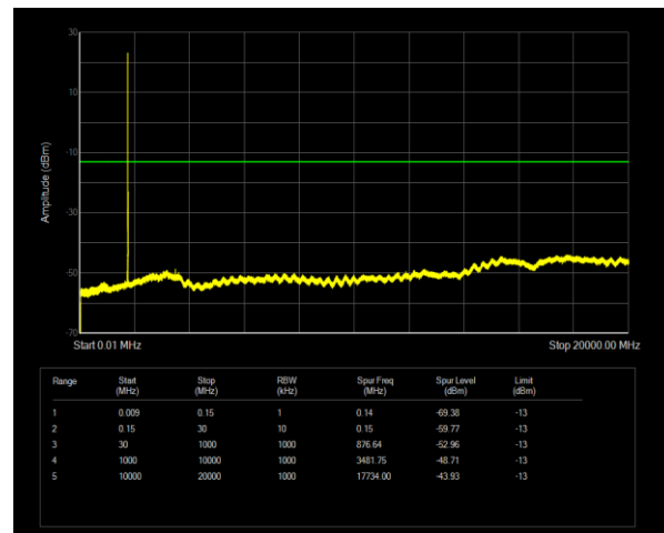
Band66 QPSK BW=10MHz Channel=132322 RB Size=1 Position=#0
