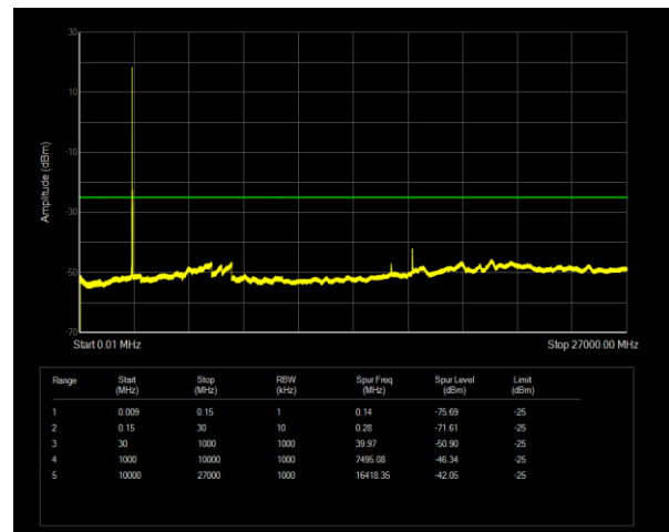
Band41(2535-2655) QPSK BW=20MHz Channel=40640 RB Size=1 Position=#0
