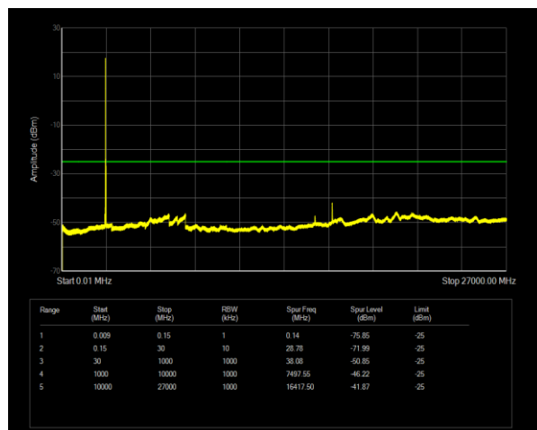
Band41(2535-2655) QPSK BW=20MHz Channel=41140 RB Size=1 Position=#0
