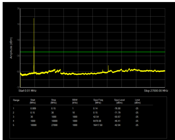
Band41(2535-2655) QPSK BW=20MHz Channel=40140 RB Size=1 Position=#0
