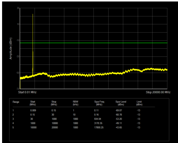
Band66 QPSK BW=15MHz Channel=132322 RB Size=1 Position=#0
