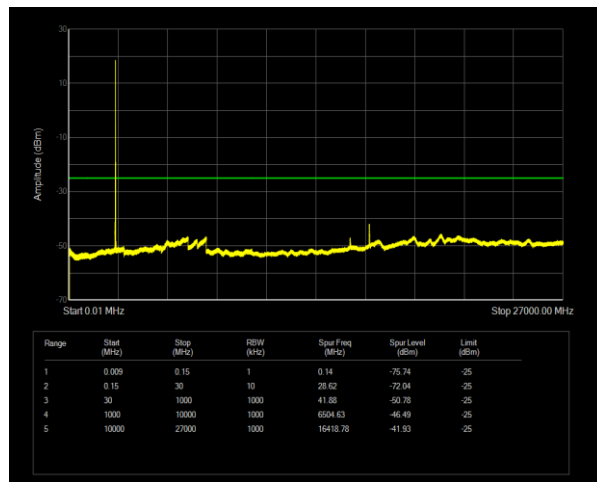
Band41(2535-2655) QPSK BW=10MHz Channel=40090 RB Size=1 Position=#0
