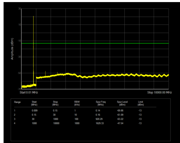
Band26(814-824) QPSK BW=5MHz Channel=26715 RB Size=1 Position=#0
