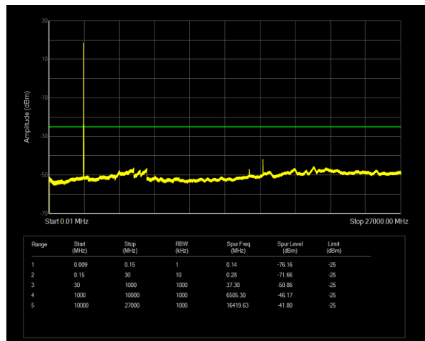
Band41(2535-2655) QPSK BW=10MHz Channel=41190 RB Size=1 Position=#0
