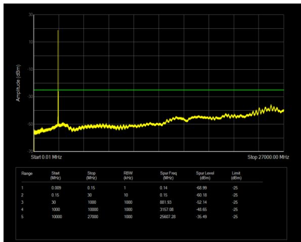
Band38 QPSK BW=20MHz Channel=38150 RB Size=1 Position=#0
