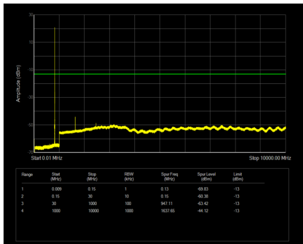
Band26(814-824) QPSK BW=1.4MHz Channel=26740 RB Size=1 Position=#0
