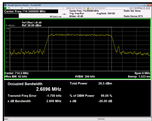
Band12 16QAM BW=3MHz Channel=23165 RB Size=15 Position=#0
