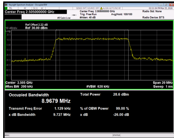
Band7 16QAM BW=10MHz Channel=20800 RB Size=50 Position=#0
