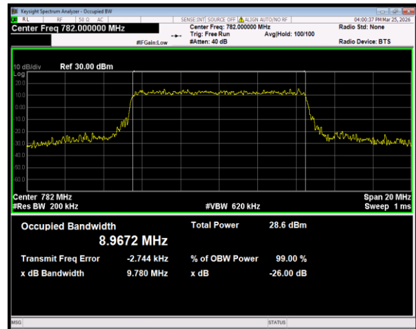
Band13 16QAM BW=10MHz Channel=23230 RB Size=50 Position=#0
