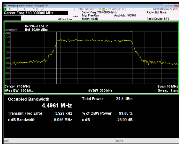
Band17 QPSK BW=5MHz Channel=23790 RB Size=25 Position=#0
