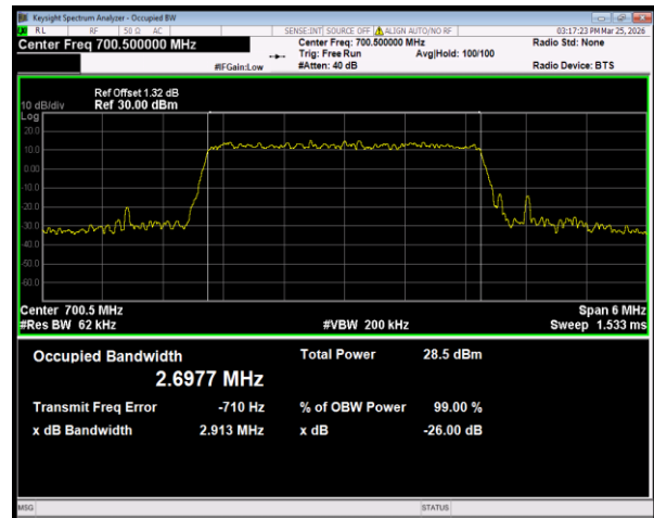
Band12 16QAM BW=3MHz Channel=23025 RB Size=15 Position=#0
