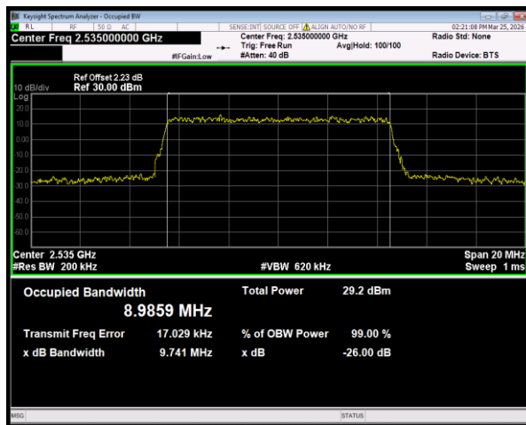
Band7 QPSK BW=10MHz Channel=21100 RB Size=50 Position=#0
