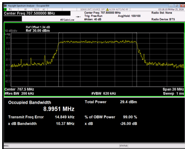
Band12 QPSK BW=10MHz Channel=23095 RB Size=50 Position=#0
