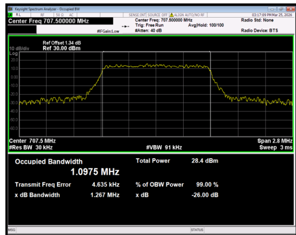
Band12 16QAM BW=1.4MHz Channel=23095 RB Size=6 Position=#0
