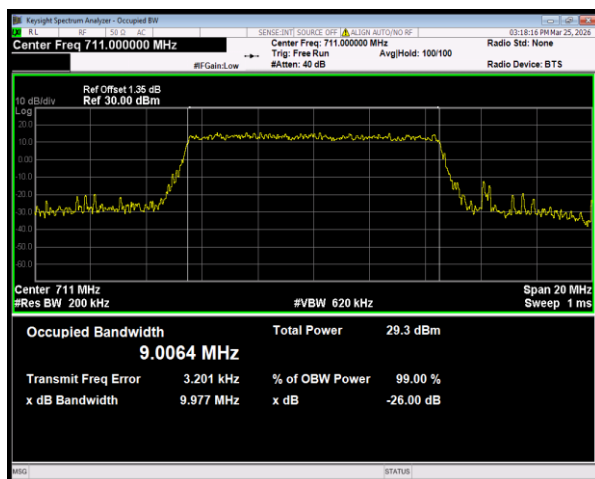
Band12 QPSK BW=10MHz Channel=23130 RB Size=50 Position=#0
