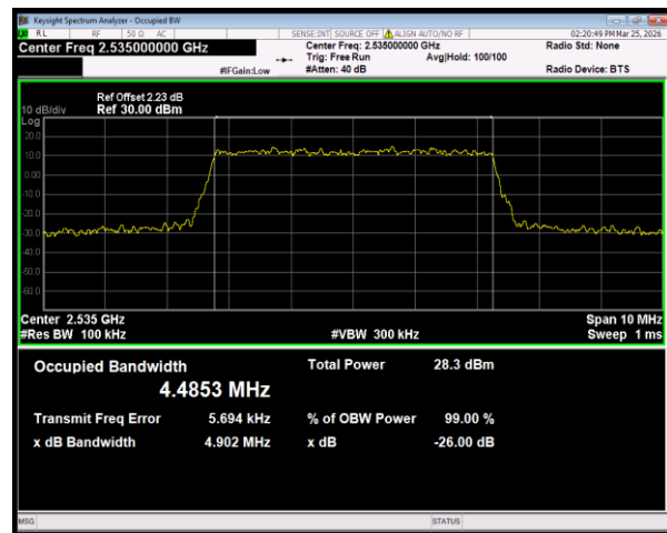
Band7 16QAM BW=5MHz Channel=21100 RB Size=25 Position=#0
