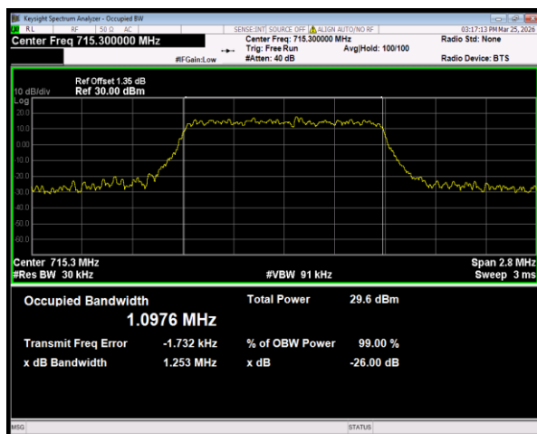
Band12 QPSK BW=1.4MHz Channel=23173 RB Size=6 Position=#0
