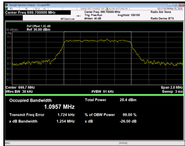
Band12 16QAM BW=1.4MHz Channel=23017 RB Size=6 Position=#0
