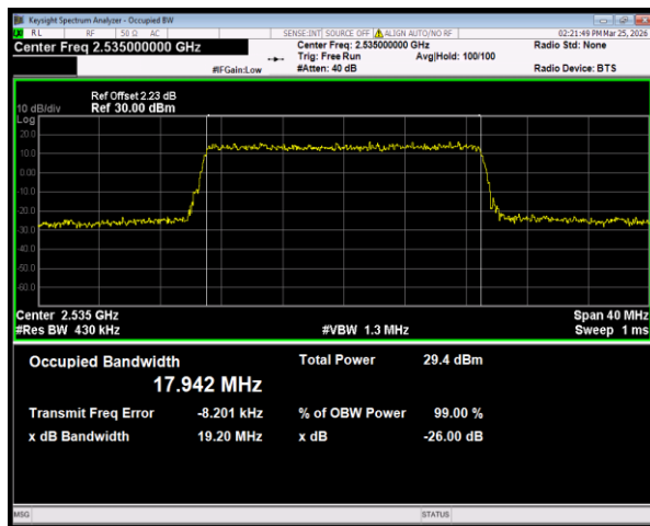
Band7 QPSK BW=20MHz Channel=21100 RB Size=100 Position=#0
