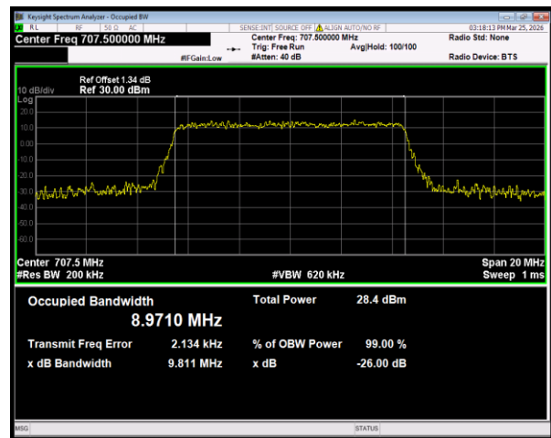
Band12 16QAM BW=10MHz Channel=23095 RB Size=50 Position=#0
