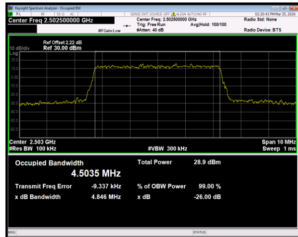
Band7 16QAM BW=5MHz Channel=20775 RB Size=25 Position=#0
