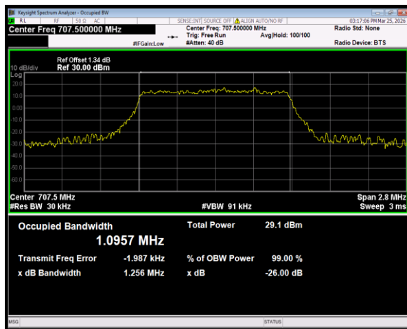
Band12 QPSK BW=1.4MHz Channel=23095 RB Size=6 Position=#0
