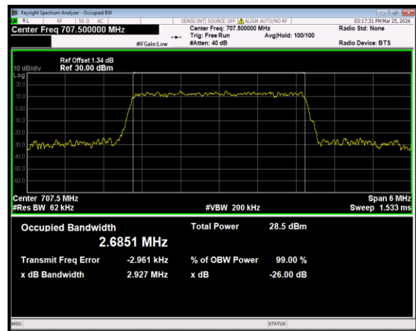
Band12 16QAM BW=3MHz Channel=23095 RB Size=15 Position=#0
