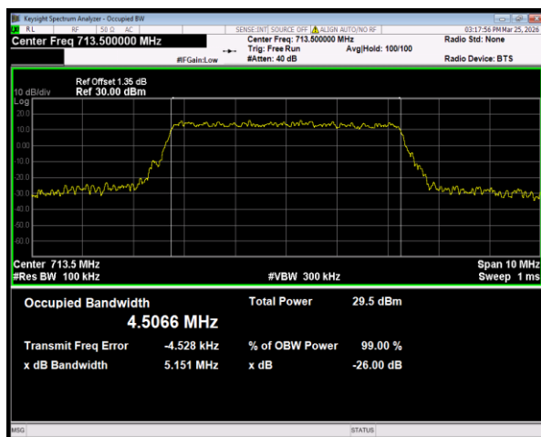
Band12 QPSK BW=5MHz Channel=23155 RB Size=25 Position=#0
