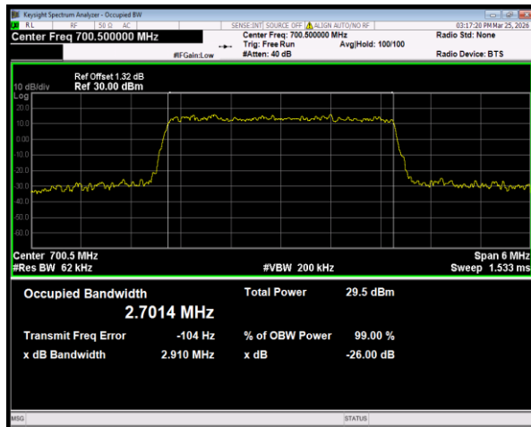
Band12 QPSK BW=3MHz Channel=23025 RB Size=15 Position=#0
