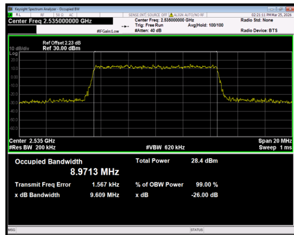
Band7 16QAM BW=10MHz Channel=21100 RB Size=50 Position=#0
