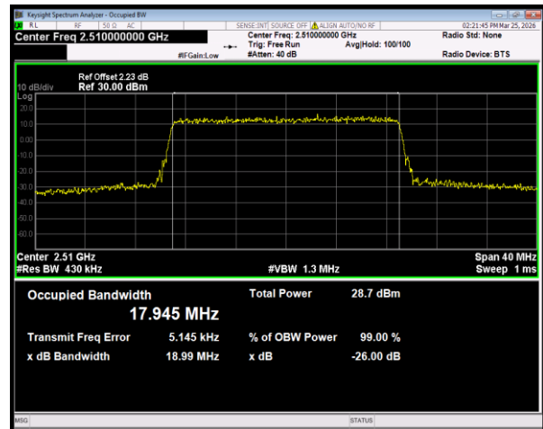
Band7 16QAM BW=20MHz Channel=20850 RB Size=100 Position=#0
