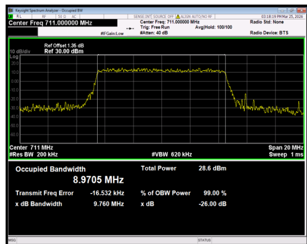
Band12 16QAM BW=10MHz Channel=23130 RB Size=50 Position=#0
