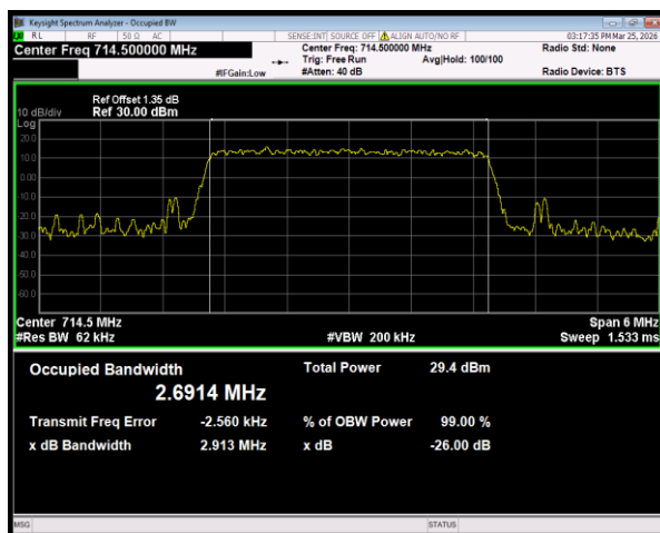
Band12 QPSK BW=3MHz Channel=23165 RB Size=15 Position=#0
