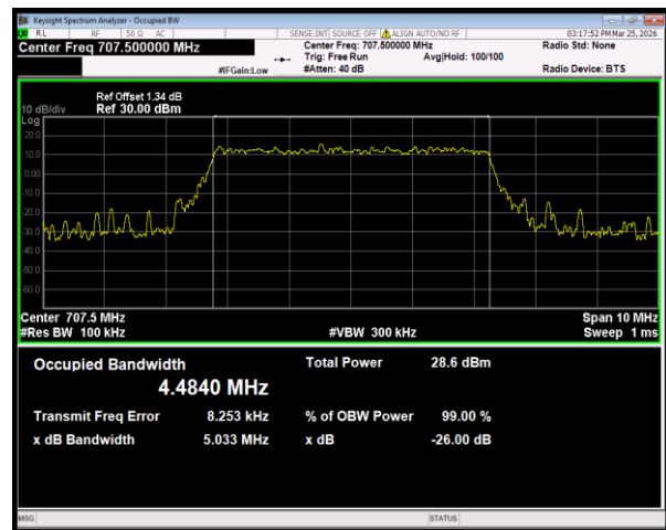
Band12 16QAM BW=5MHz Channel=23095 RB Size=25 Position=#0
