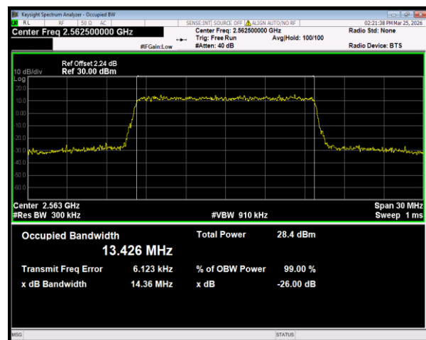
Band7 16QAM BW=15MHz Channel=21375 RB Size=75 Position=#0
