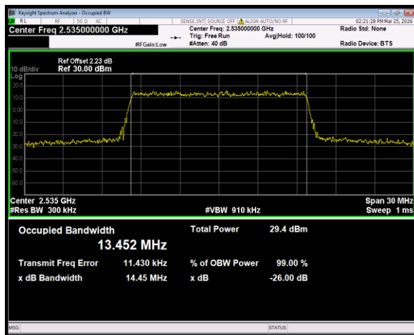
Band7 QPSK BW=15MHz Channel=21100 RB Size=75 Position=#0
