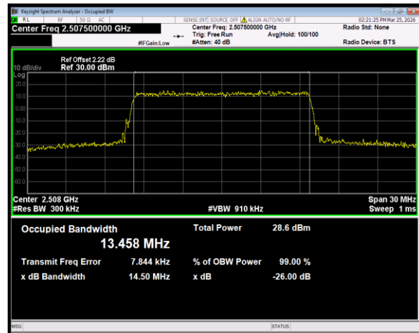
Band7 16QAM BW=15MHz Channel=20825 RB Size=75 Position=#0
