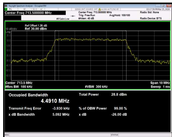
Band12 16QAM BW=5MHz Channel=23155 RB Size=25 Position=#0
