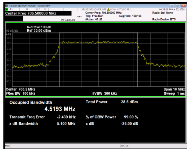
Band17 16QAM BW=5MHz Channel=23755 RB Size=25 Position=#0
