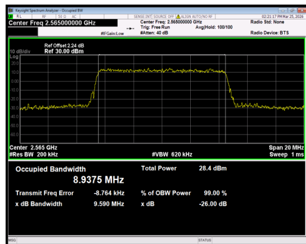
Band7 16QAM BW=10MHz Channel=21400 RB Size=50 Position=#0
