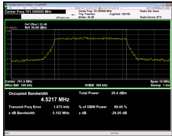
Band12 16QAM BW=5MHz Channel=23035 RB Size=25 Position=#0
