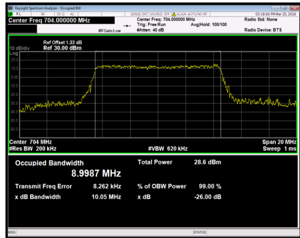
Band12 16QAM BW=10MHz Channel=23060 RB Size=50 Position=#0
