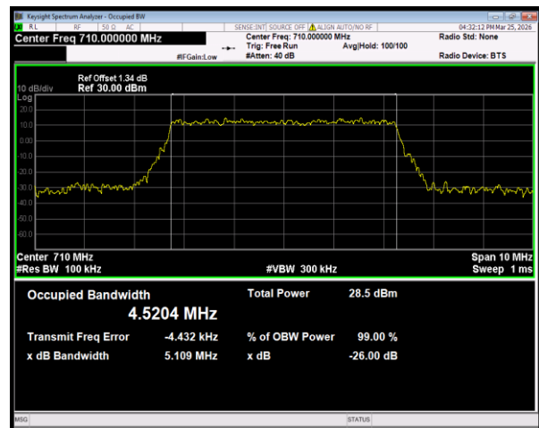
Band17 16QAM BW=5MHz Channel=23790 RB Size=25 Position=#0
