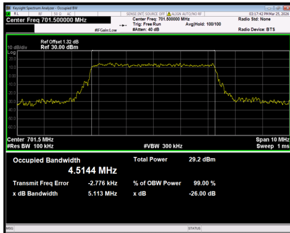
Band12 QPSK BW=5MHz Channel=23035 RB Size=25 Position=#0
