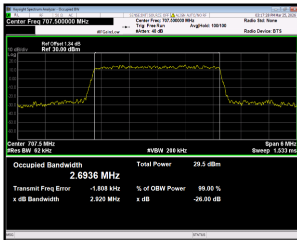
Band12 QPSK BW=3MHz Channel=23095 RB Size=15 Position=#0
