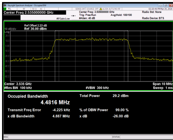
Band7 QPSK BW=5MHz Channel=21100 RB Size=25 Position=#0
