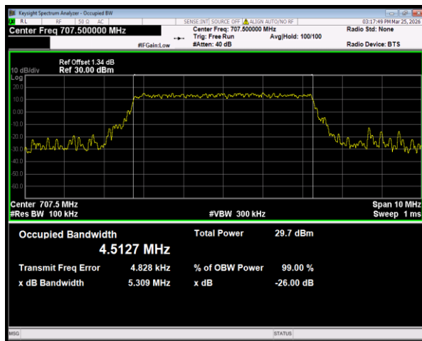
Band12 QPSK BW=5MHz Channel=23095 RB Size=25 Position=#0
