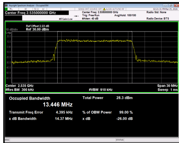
Band7 16QAM BW=15MHz Channel=21100 RB Size=75 Position=#0
