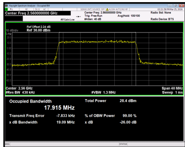
Band7 16QAM BW=20MHz Channel=21350 RB Size=100 Position=#0
