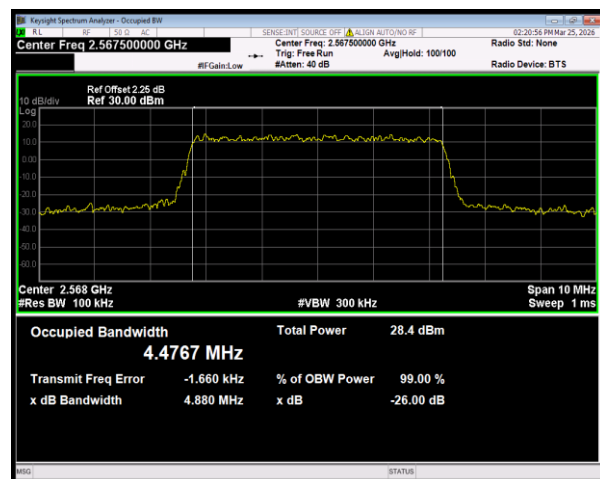
Band7 16QAM BW=5MHz Channel=21425 RB Size=25 Position=#0
