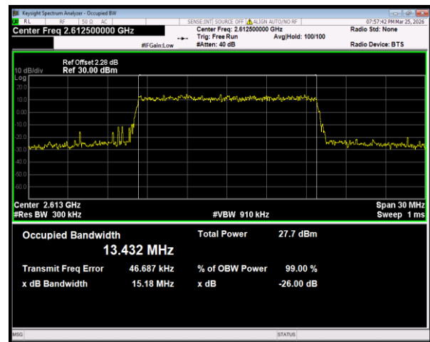
Band38 16QAM BW=15MHz Channel=38175 RB Size=75 Position=#0
