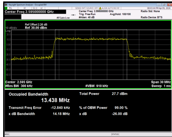
Band41(2535-2655) 16QAM BW=15MHz Channel=40640 RB Size=75 Position=#0
