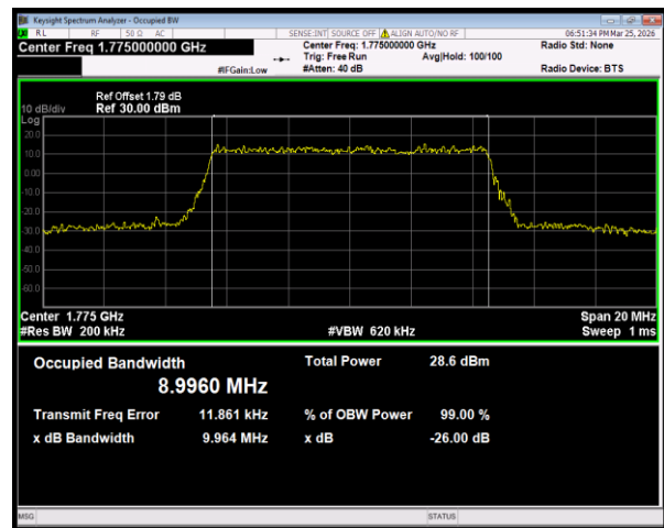
Band66 16QAM BW=10MHz Channel=132622 RB Size=50 Position=#0
