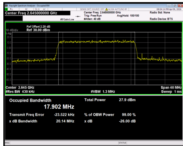
Band41(2535-2655) 16QAM BW=20MHz Channel=41140 RB Size=100 Position=#0
