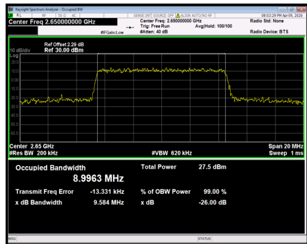
Band41(2535-2655) 16QAM BW=10MHz Channel=41190 RB Size=50 Position=#0
