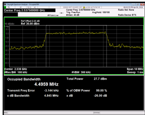
Band41(2535-2655) 16QAM BW=5MHz Channel=40065 RB Size=25 Position=#0
