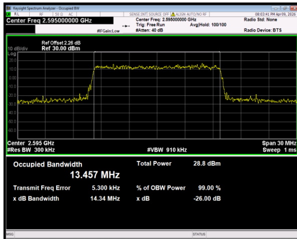
Band41(2535-2655) QPSK BW=15MHz Channel=40640 RB Size=75 Position=#0
