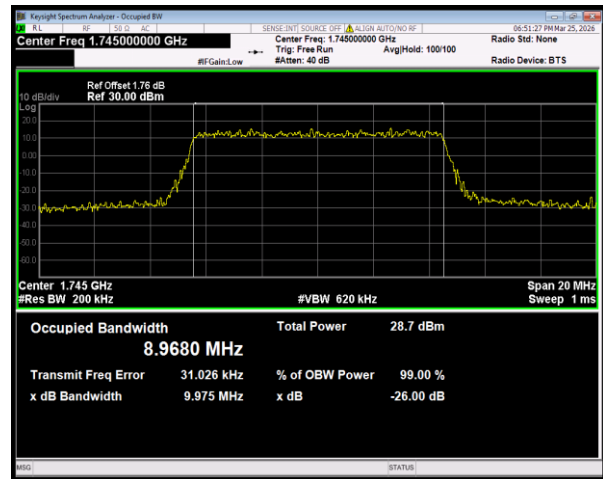
Band66 16QAM BW=10MHz Channel=132322 RB Size=50 Position=#0
