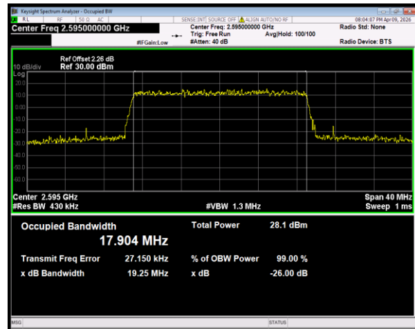
Band41(2535-2655) 16QAM BW=20MHz Channel=40640 RB Size=100 Position=#0
