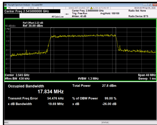
Band41(2535-2655) 16QAM BW=20MHz Channel=40140 RB Size=100 Position=#0
