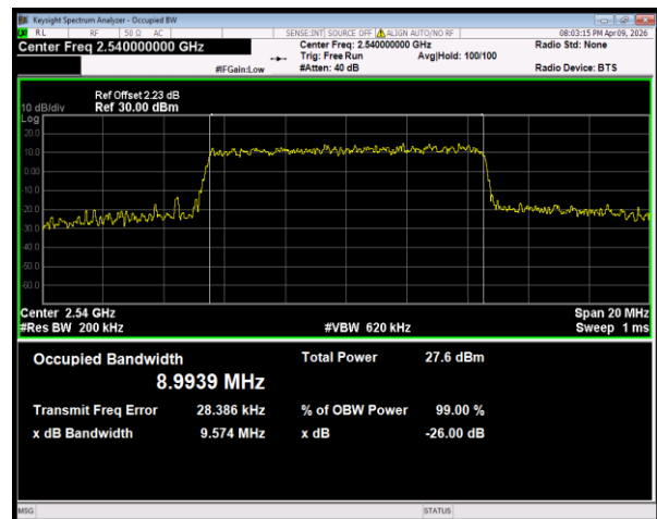
Band41(2535-2655) 16QAM BW=10MHz Channel=40090 RB Size=50 Position=#0
