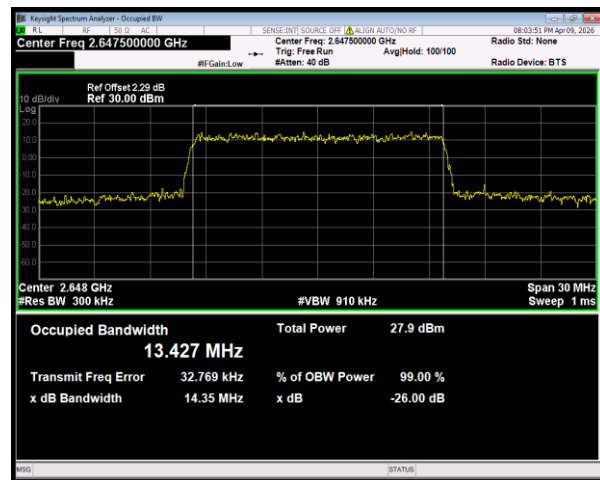
Band41(2535-2655) 16QAM BW=15MHz Channel=41165 RB Size=75 Position=#0
