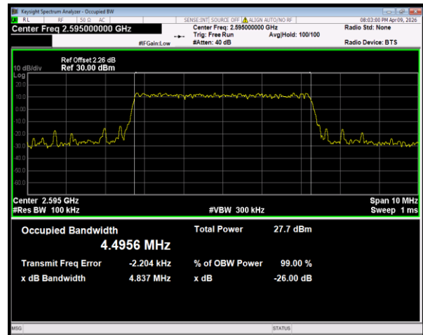
Band41(2535-2655) 16QAM BW=5MHz Channel=40640 RB Size=25 Position=#0
