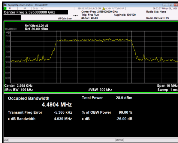
Band41(2535-2655) QPSK BW=5MHz Channel=40640 RB Size=25 Position=#0
