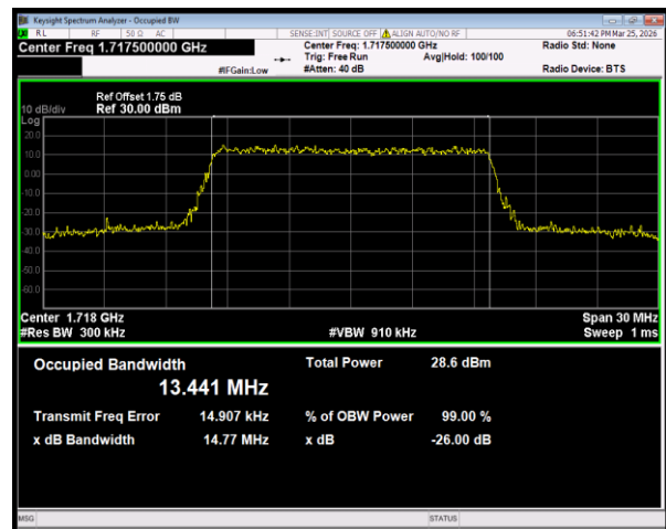
Band66 16QAM BW=15MHz Channel=132047 RB Size=75 Position=#0
