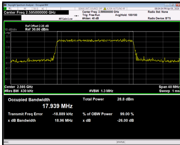
Band41(2535-2655) QPSK BW=20MHz Channel=40640 RB Size=100 Position=#0
