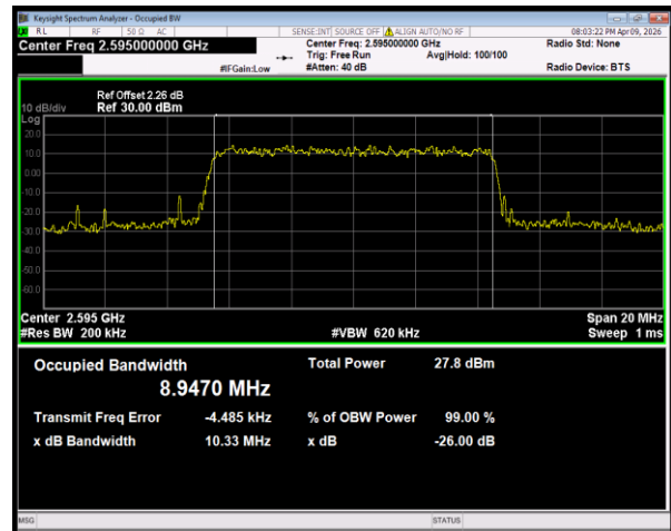
Band41(2535-2655) 16QAM BW=10MHz Channel=40640 RB Size=50 Position=#0
