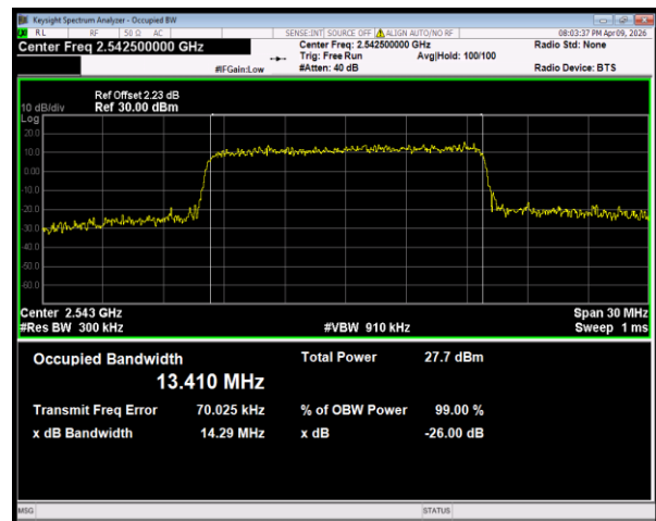
Band41(2535-2655) 16QAM BW=15MHz Channel=40115 RB Size=75 Position=#0
