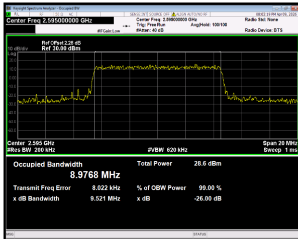
Band41(2535-2655) QPSK BW=10MHz Channel=40640 RB Size=50 Position=#0
