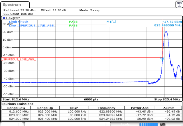
1.4MHz_Low_QPSK_1@0 -17.72dBm
