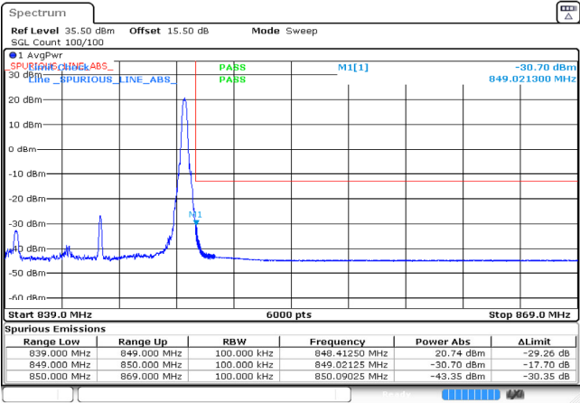
10MHz_High_QPSK_1@49 -30.70dBm
