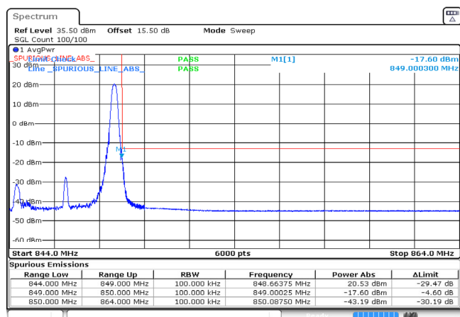
5MHz_High_QPSK_1@24 -17.60dBm
