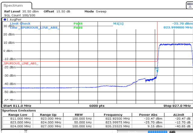
3MHz_Low_QPSK_15@0 -25.70dBm
