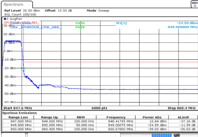
1.4MHz_High_QPSK_6@0 -24.59dBm
