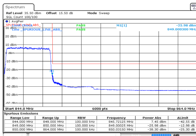
5MHz_High_QPSK_25@0 -25.98dBm
