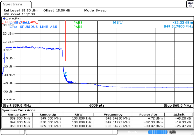
10MHz_High_QPSK_50@0 -32.33dBm
