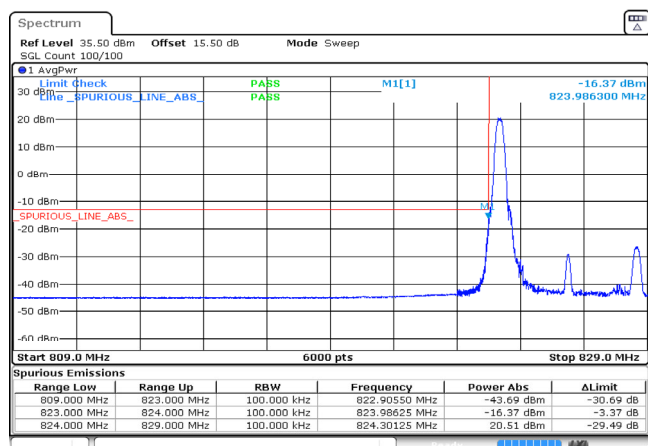
5MHz_Low_QPSK_1@0 -16.37dBm
