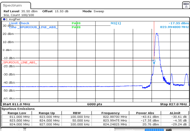
3MHz_Low_QPSK_1@0 -17.35dBm
