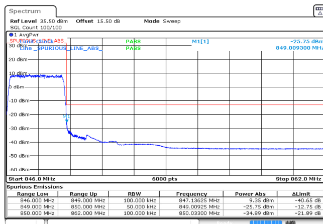
3MHz_High_QPSK_15@0 -25.75dBm
