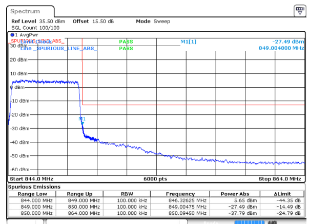
5MHz_High_16QAM_25@0
