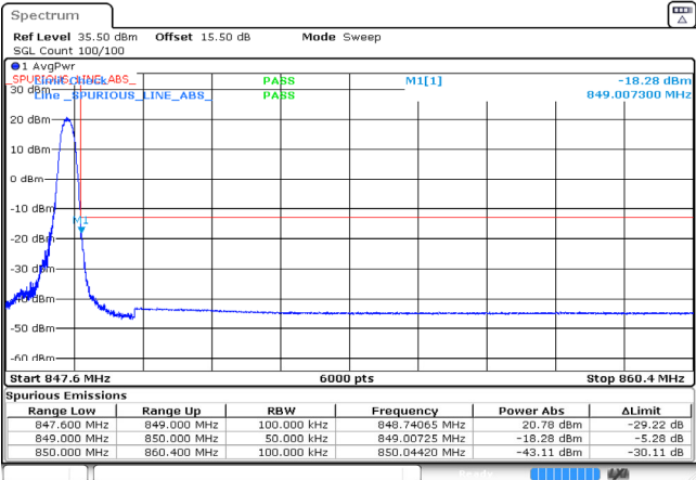
1.4MHz_High_QPSK_1@5 -18.28dBm
