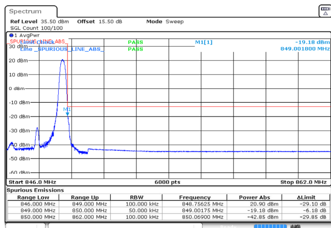
3MHz_High_QPSK_1@14 -19.18dBm
