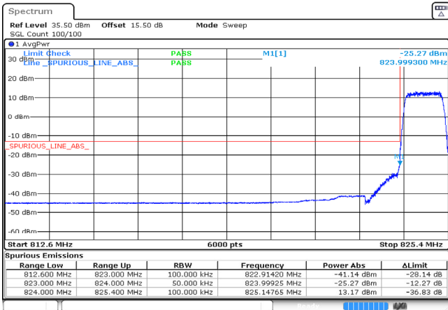
1.4MHz_Low_QPSK_6@0 -25.27dBm
