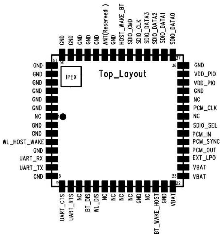
Figure 2: GOC-RG440-WZ Pin
