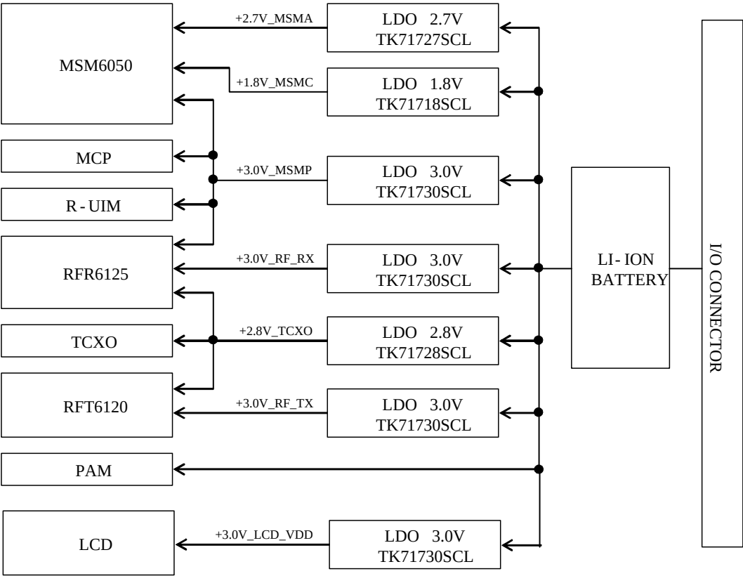
BCL862S Power Part Block Diagram
