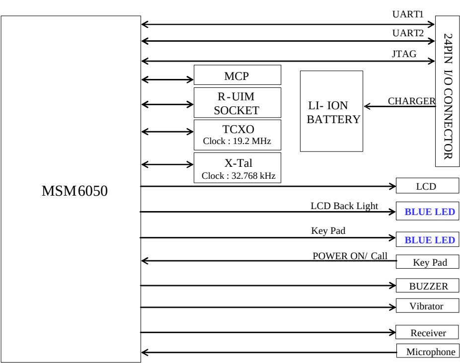
BCL862S Logic Part Block Diagram
