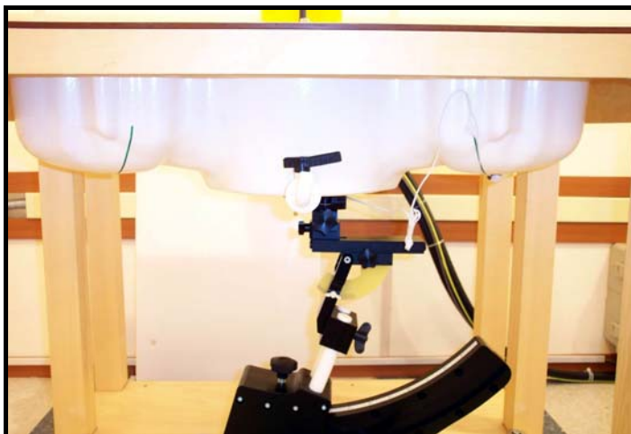
Figure 9.6 Muscle SAR Test Setup -- 15mm Distance with headset Position --
