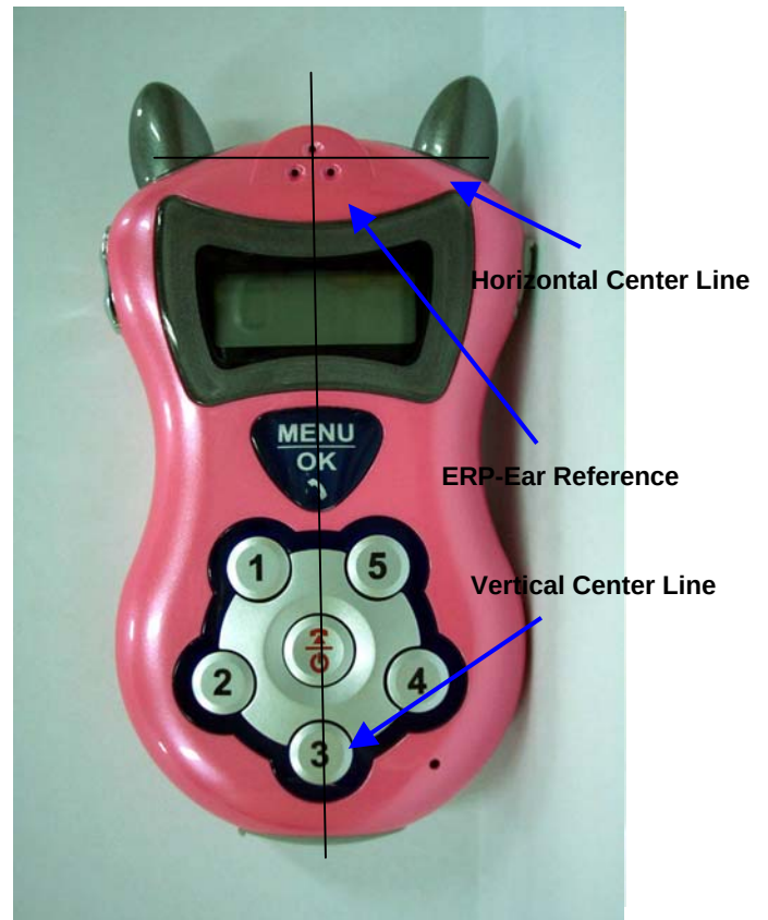
Figure 9.1 Handset Reference Points
