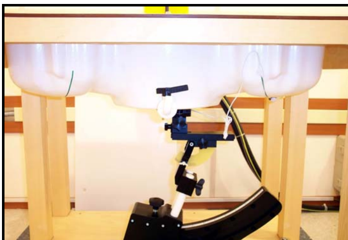
Figure 9.6 Muscle SAR Test Setup -- Touch Position with headset --
