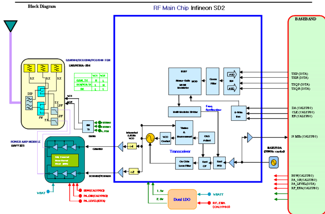
Figure 2 Transmitter Block Diagram
