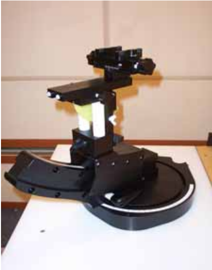
Figure 3.6Device Holder
