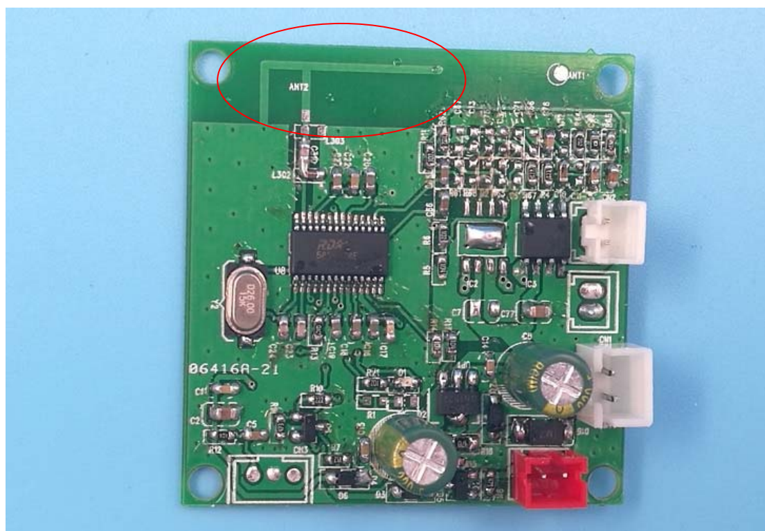
4. BT antenna view
