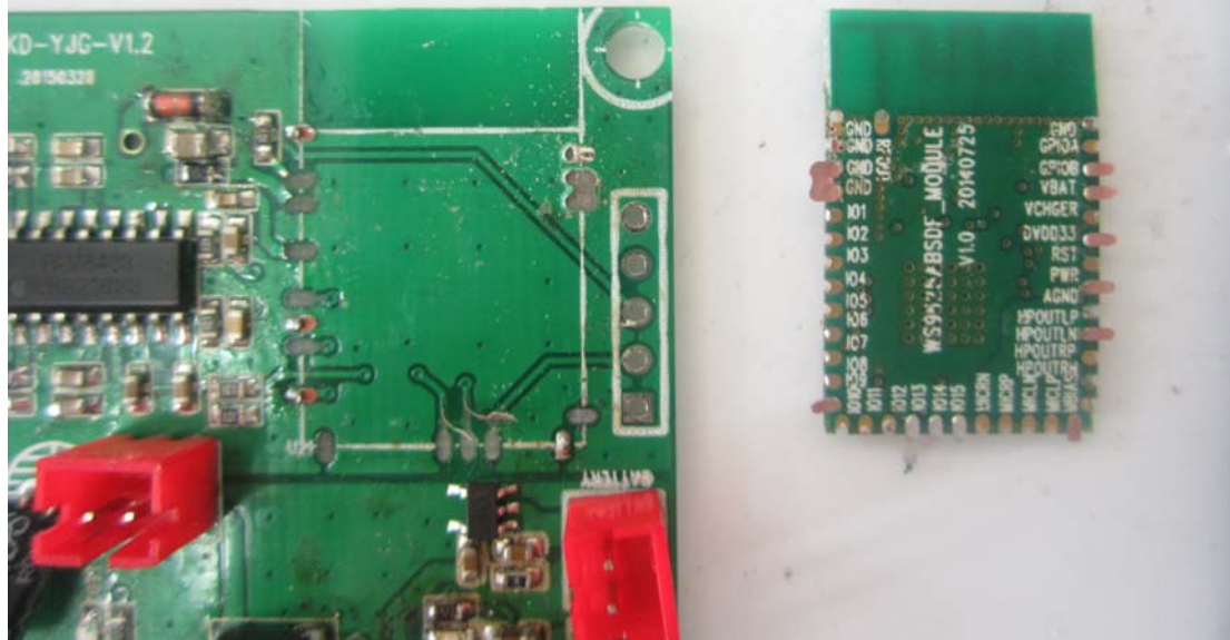
3. Mainboard rear view
