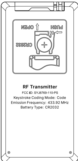
Back cover screen print location drawing
