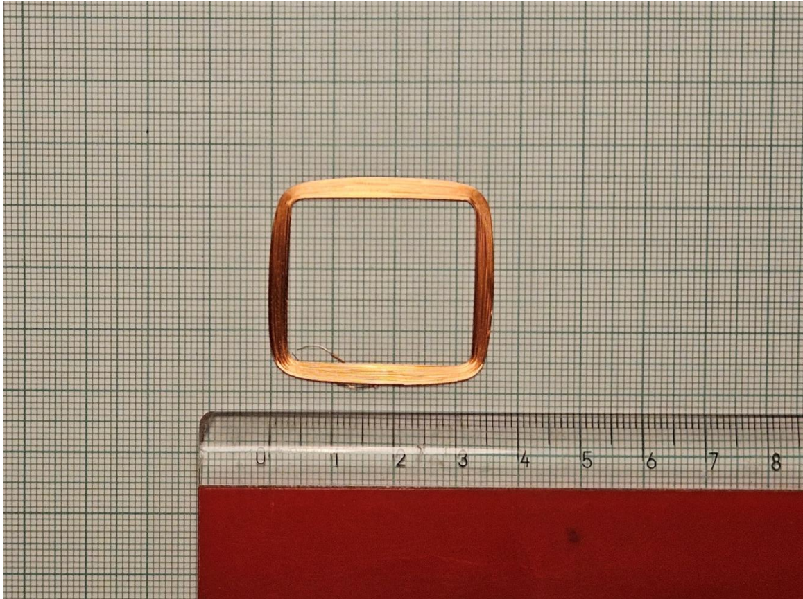
Antenna 125 kHz
